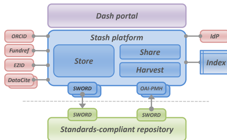
Figure 6. Dash high-level architecture.
