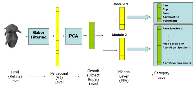
Figure 4: Image Preprocessing.
