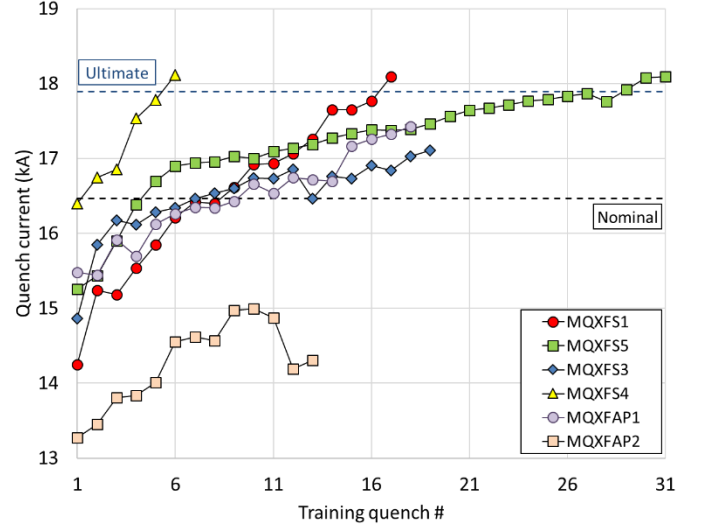
Fig. 18. Comparison of quench current during training of the first thermal cycle of tested magnets, at 1.9 K and 20 A/s. Quenches of MQXFAS3 are plotted only up to the maximum current before degradation. Data are compared to nominal, ultimate and short-sample current (estimated from witness samples).
