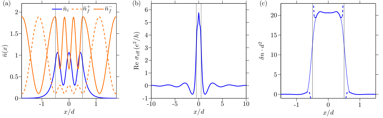
FIG. S1. (a) The normalized density distribution \bar{n} of the wave functions in a bound-to-continuum optical transition for U \equiv ud/\hbar v_F = 5 , K_y \equiv k_y d = 5 and \omega d/v_F = 1.7 . The bound state density (blue) is localized at the well, while the continuum state densities (orange) are extended. The bound state is on the m = 3 branch and has even parity, thus transition into the even parity final state (dashed curve) is forbidden. The vertical dotted lines indicate the boundaries of the square well. (b) The real part of the effective conductivity calculated with the same parameters as in (a) and E_F = 4 . The peak at the center is caused by bound-to-continuum state transitions, while the long range oscillations with wavevector \omega/v_F come from the transitions between states in the continuum. (c) Density perturbation induced by a square well of depth U = 5 at E_F = 4 . The step-like discontinuity in the potential leads to a 1/x divergence at the edges of the well, shown by the dashed curves. For any realistic smooth potential the divergence is regularized, as shown schematically by the thin solid curves.
