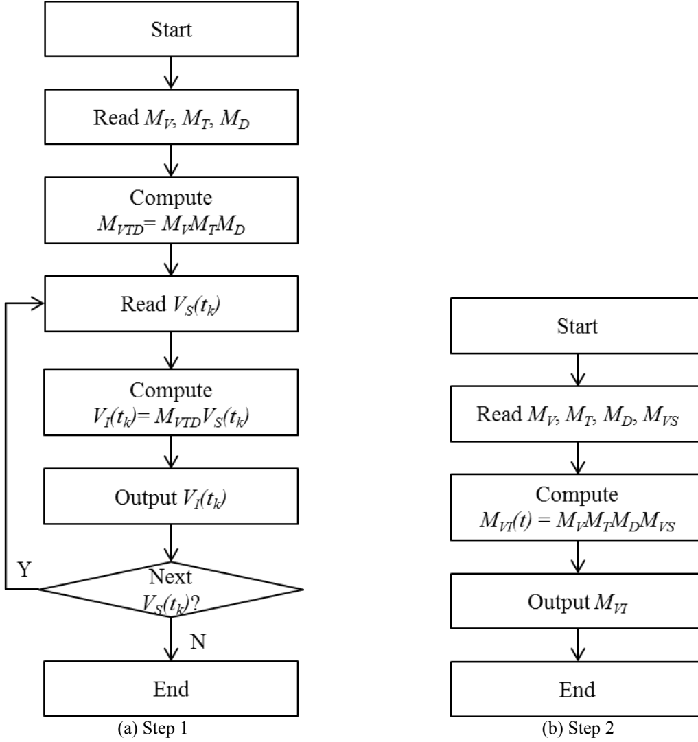
Figure 10. Optimization of the Radiance daylighting simulation algorithm
