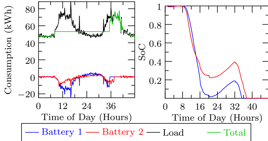
Figure 3.18: Optimal solution for quadratic pricing with linear battery model
