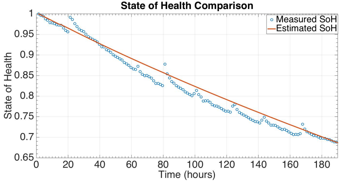
Figure 3.15: SoH profiles of measured data and model output.
