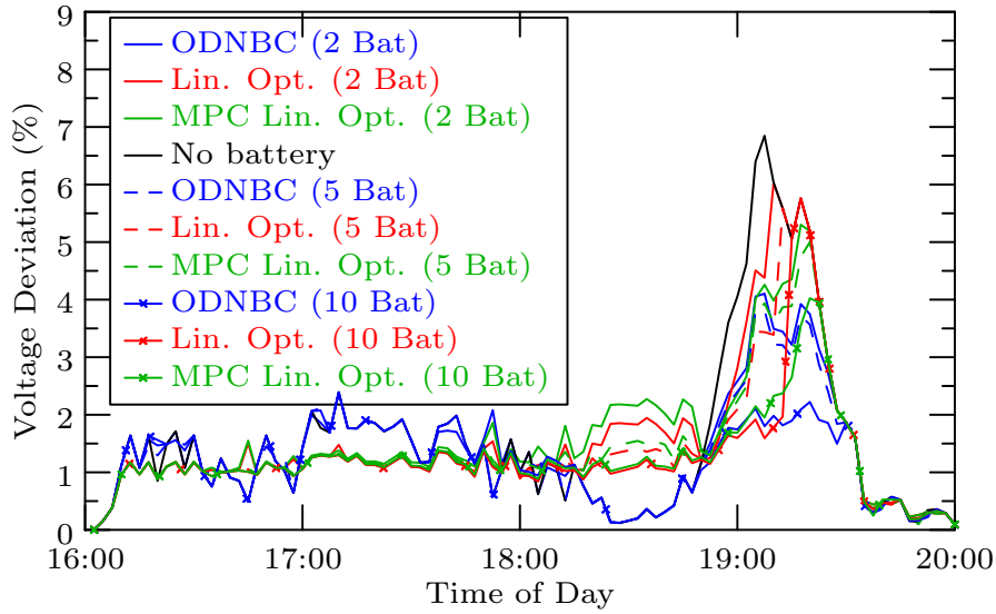
Figure 3.32: Absolute voltage deviation profile comparison of all solutions.
