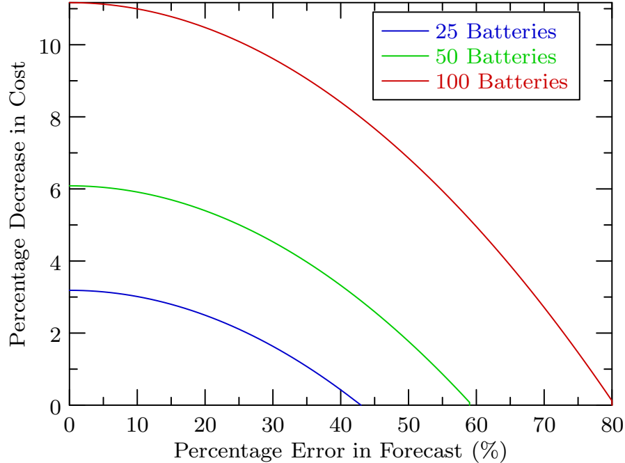
Figure 3.29: Percentage decrease in electricity cost with respect to the no-battery case for the research building
