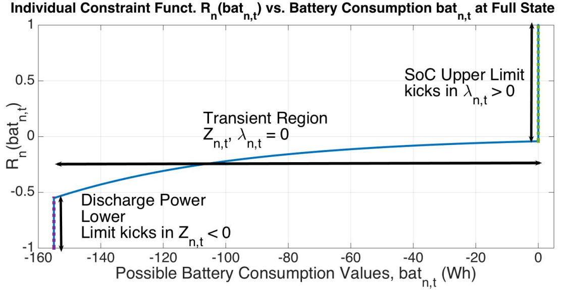
Figure 3.3: Optimal solutions at a single time step for a full battery. The battery cannot be charged further and the individual constraint function is dominated by \lambda_{n,t} on the positive side and by Z_{n,t} on the negative side.
