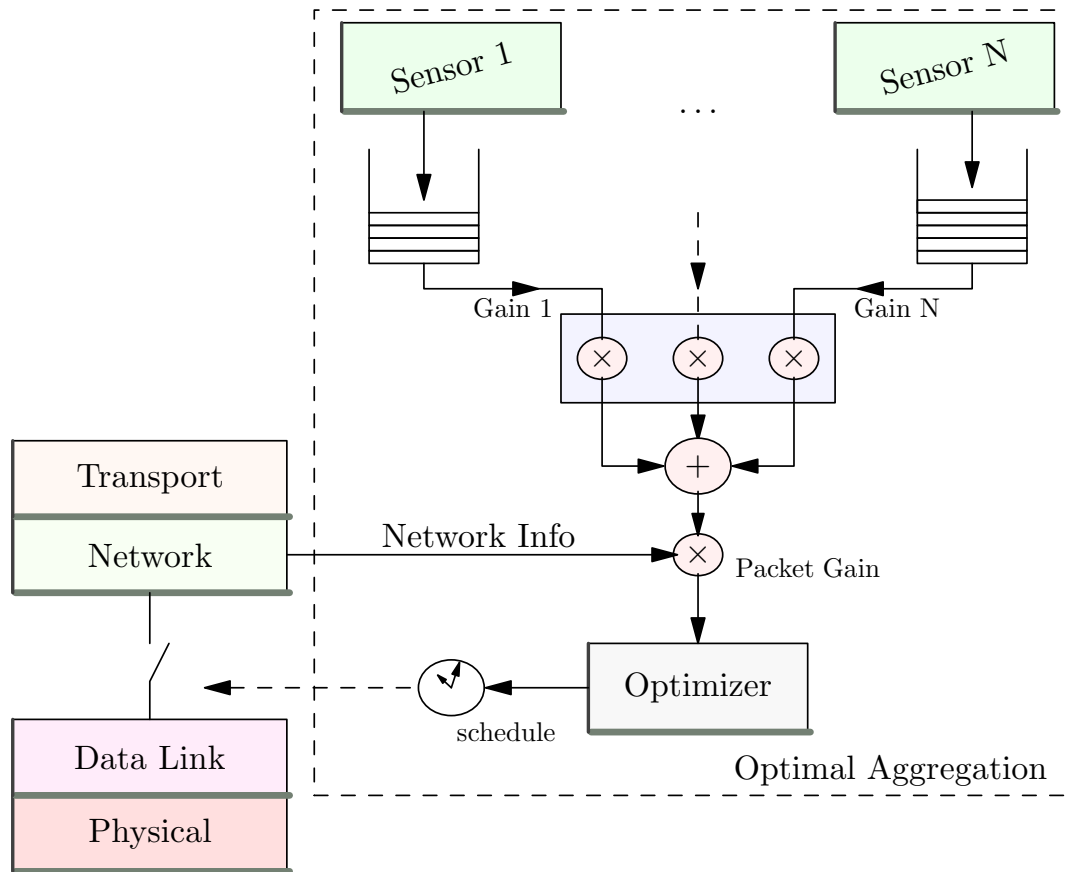
Figure 5.1: Architecture of our solution within a single node.
