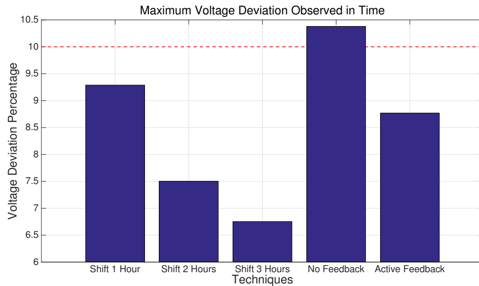
Figure 4.11: System stability of the neighborhood case study
