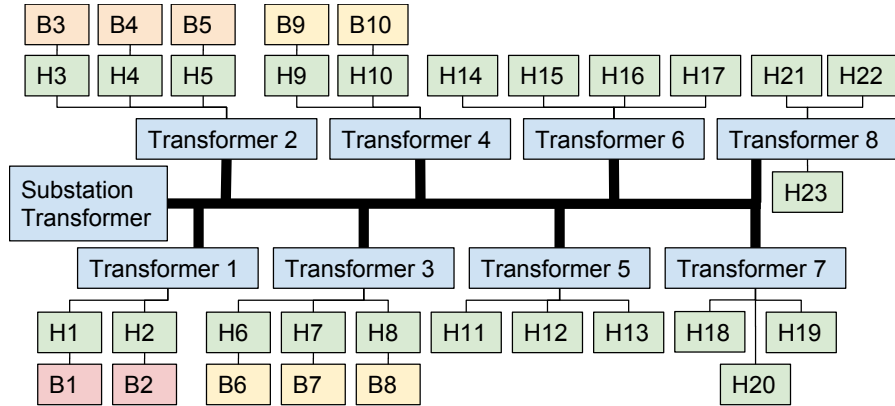
Figure 3.31: Neighborhood circuit with battery locations
