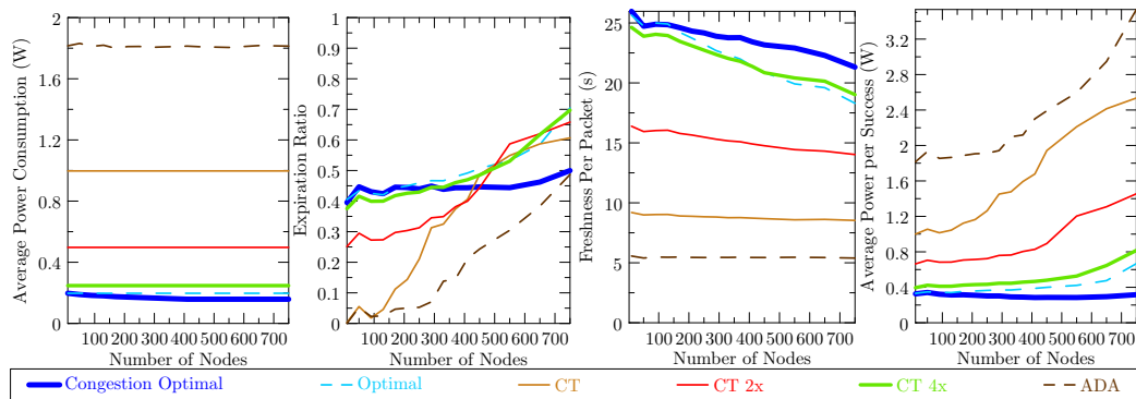
Figure 5.10: San Diego Downtown case with two streams on each node. Number of nodes is increased to observe the effect of congestion.
