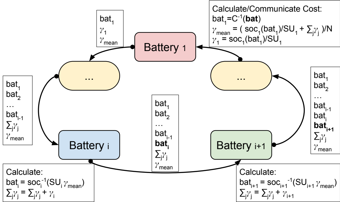
Figure 3.10: The mean circular negotiation ring illustration, where each node calculates their consumption based on the mean \gamma ratio from the previous iteration.
