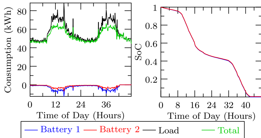
Figure 3.17: Optimal solution for quadratic pricing with nonlinear battery model
