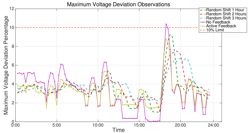
Figure 4.10: Neighborhood case study with distributed heterogeneous controls
