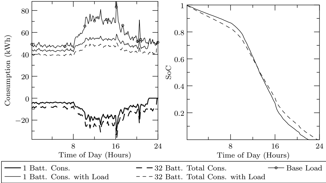
Figure 3.23: 24 hour solution time series for single battery and 32 batteries cases.
