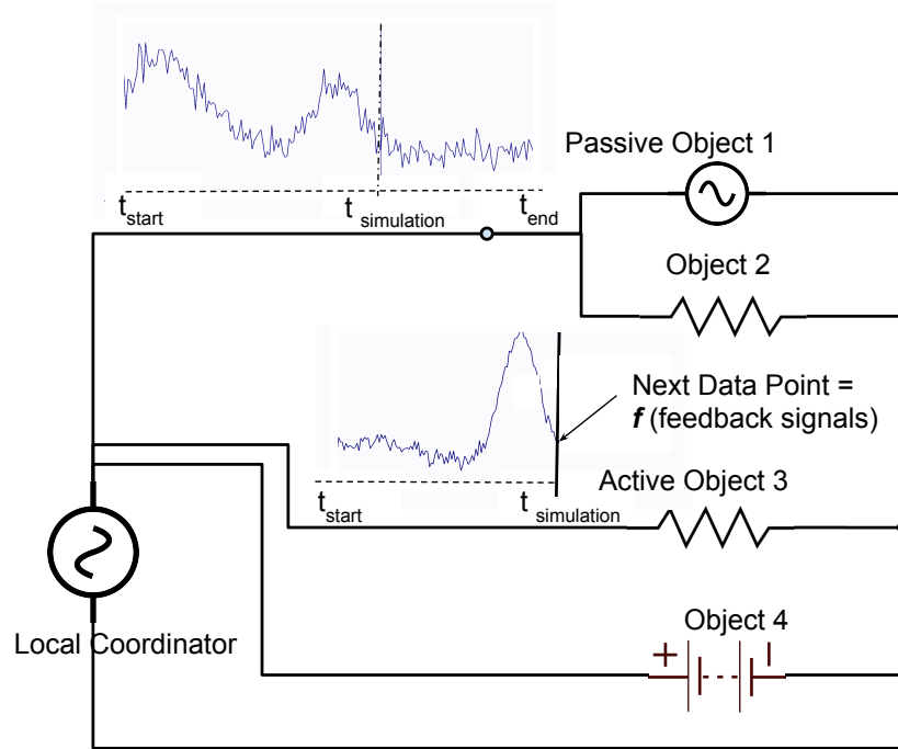
Figure 4.5: Example circuit with passive and active connections
