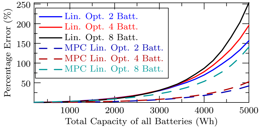
Figure 3.27: Error of linear model solutions, compared to our optimal solution.
