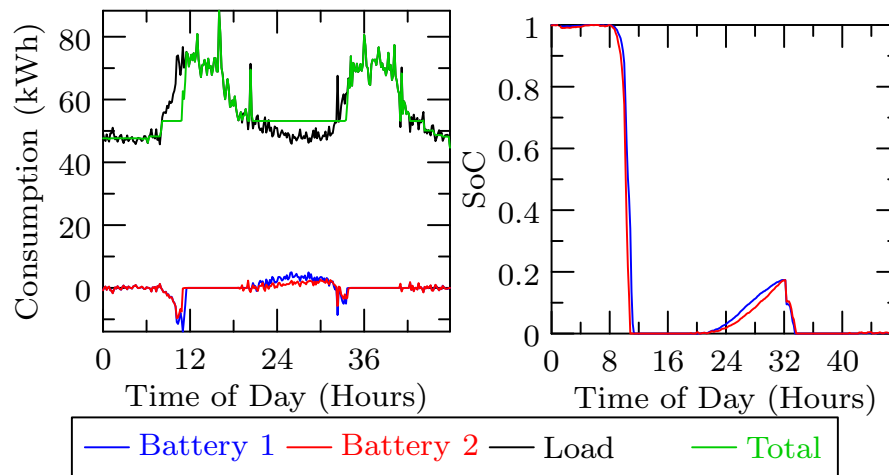
Figure 3.21: Linear optimal solution for quadratic pricing with a lossy nonlinear battery
