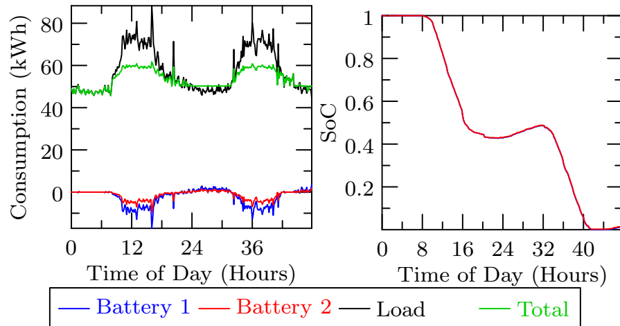
Figure 3.19: Optimal solution for fourth order pricing with nonlinear battery model
