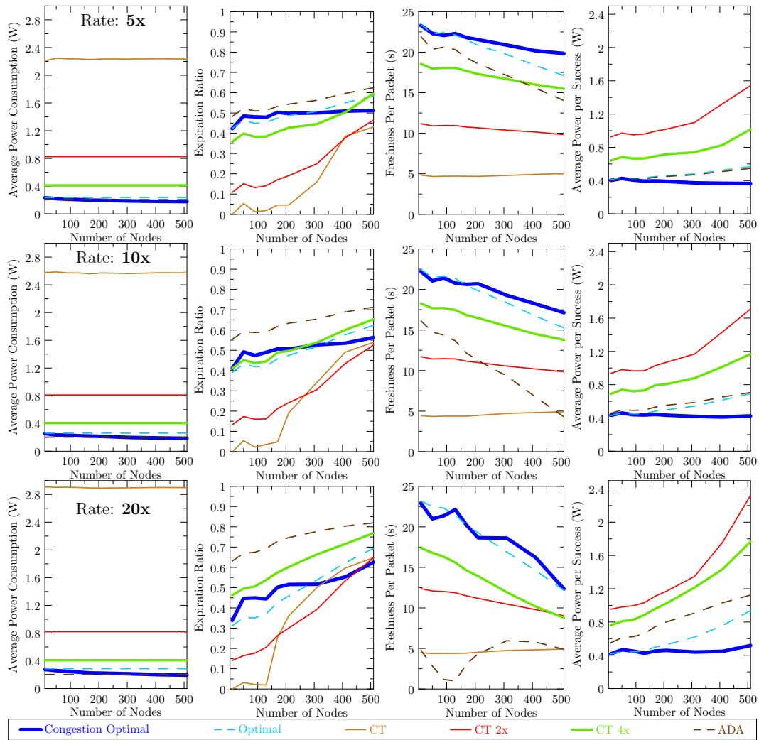
Figure 5.11: San Diego Downtown case with two varying speed streams on each node. Number of nodes is increased to observe the effect of congestion. The top four figures are for the 5x case, middle four figures are 10x and bottom four figures are 20x.
