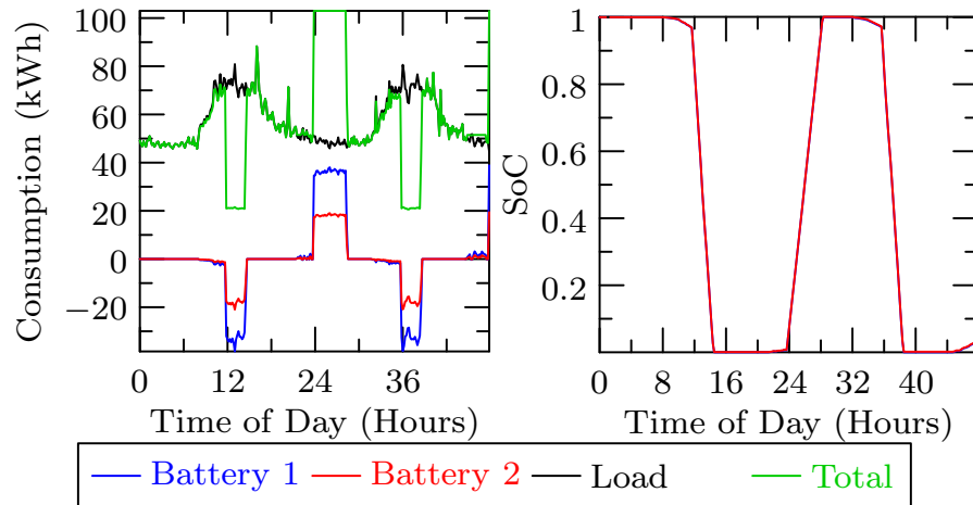
Figure 3.16: Optimal solution for a time of use pricing with nonlinear battery model
