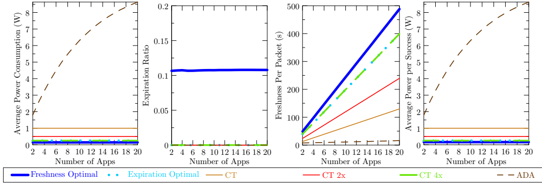
Figure 5.5: Effect of number of application streams on performance. Information freshness increases linearly with the number of streams since more data can be aggregated onto packets, while the expiration rate and power consumption stay constant as the period stays constant. Expiration Optimal and CT 4x have the same period, thus their results are overlapping. In the expiration ratio figure, only Freshness Optimal result has a non-zero expiration rate.
