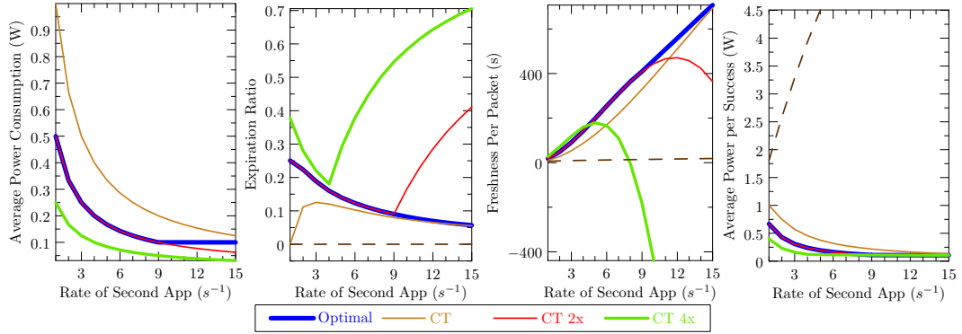
Figure 5.4: Combination of heterogeneous application streams. As the generation rate of the second application stream increases, the weighted average of the gain functions favors towards the second stream. The power consumption is not shown for ADA as it grows very fast relative to the other solutions. However, it is observable in the average power per success figure, since its success rate is 1.
