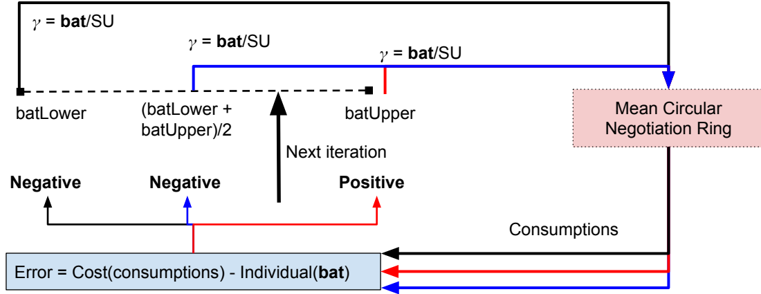
Figure 3.12: The bisection method workflow illustration.
