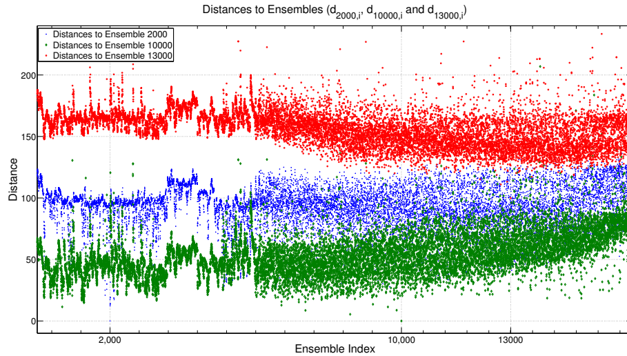
Figure 2.2: The euclidean distance of all sorted ensembles to the Ensemble 2000 (blue), Ensemble 10000 (green) and Ensemble 13000 (red).
