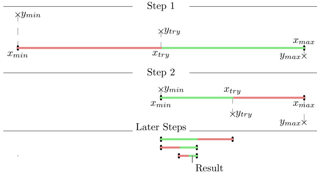
Figure 5.2: An example for the Bisection Method. The interval is divided into half at each iteration, making the search interval smaller every time. The algorithm stops, when the desired solution resolution is achieved.
