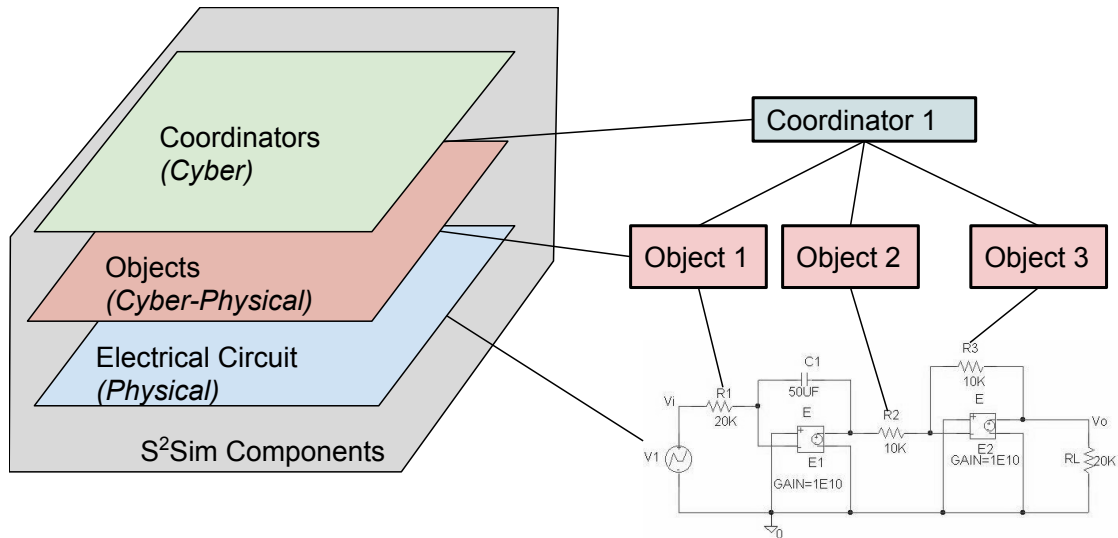
Figure 4.2: CPS Layers of S 2 Sim.
