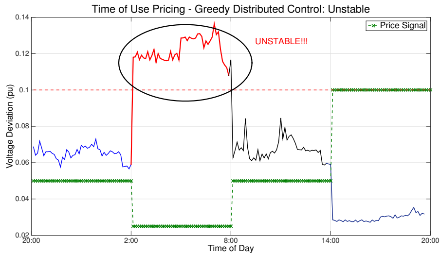
Figure 4.6: Time of Use Pricing resulting in unstable system behavior
