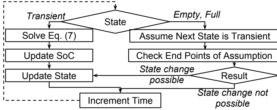
Figure 3.7: Algorithm flowchart for the centralized solution.
