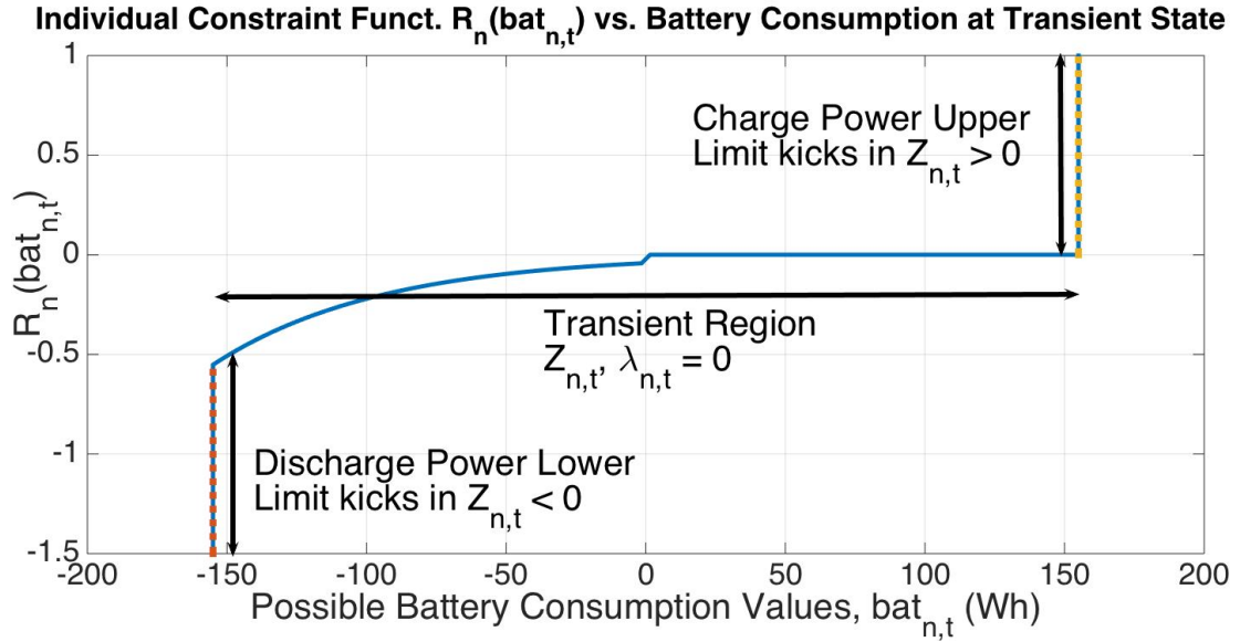
Figure 3.4: Optimal solutions at a single time step for a transient state battery, neither full nor empty. The battery is limited by the power limits and the individual constraint function is dominated by Z_{n,t} on both limits.
