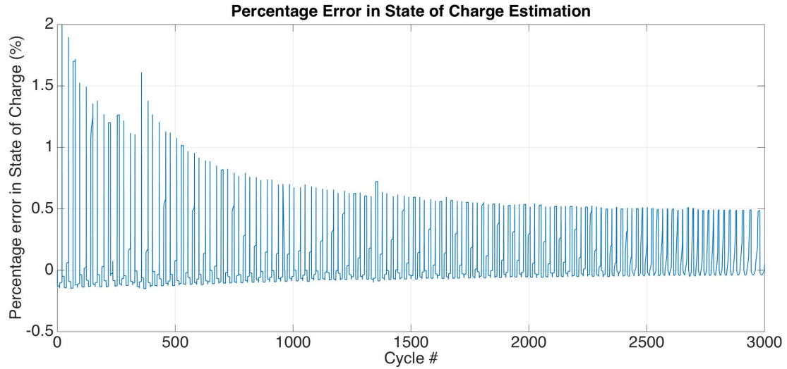
Figure 3.14: State of charge error percentage profile of the model's output.
