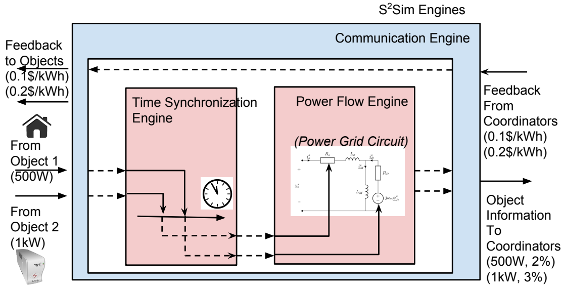
Figure 4.3: Functionalities of S 2 Sim divided among its internal components.
