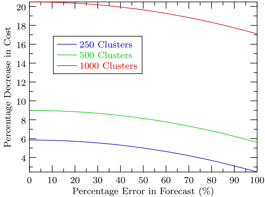
Figure 3.30: Percentage decrease in electricity cost with respect to the no-battery case for the medical institution
