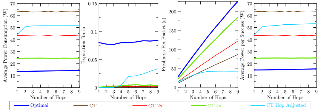
Figure 5.12: Multi-hop simulation results for the linear topology are given to study the additional effects of forwarding delays.
