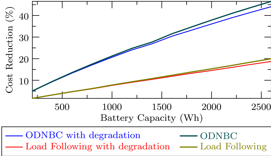
Figure 3.22: Cost reduction in electricity bill for ODNBC and load following.
