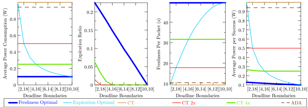
Figure 5.3: Effect of deadline randomness on the performance. Our freshness optimal solution has the highest information freshness, lowest energy consumption and lowest energy per non-expired data, while our expiration optimal solution has no expiration.
