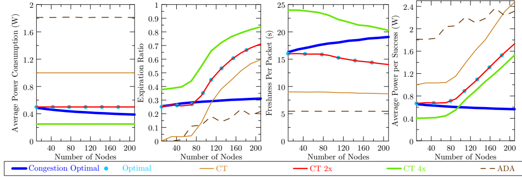
Figure 5.8: 5G RAN heterogeneous gain function simulation results. Stream 1: 1s^{-1} rate, information freshness gain function, 1s deadline. Stream 2: 1s^{-1} rate, expiration gain function, 9s deadline. Optimal and CT 2x cases have the same period, thus the results are overlapping.
