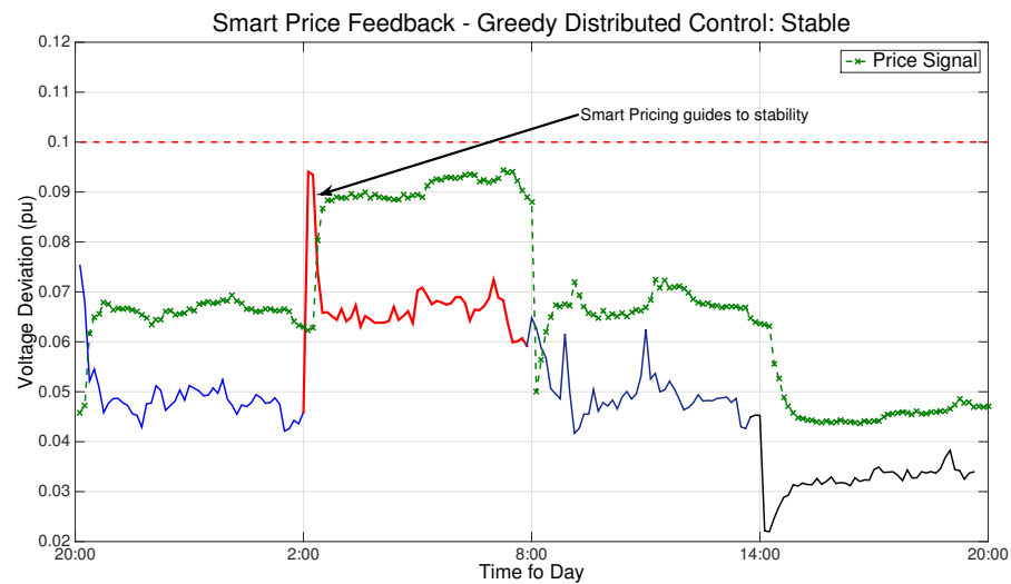
Figure 4.7: Adaptive Pricing resulting in stable system behavior
