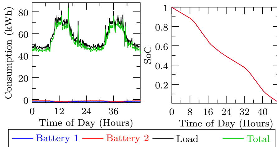
Figure 3.20: Optimal solution for quadratic pricing with lossy nonlinear battery model
