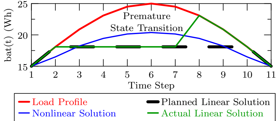
Figure 3.26: Example of linear model assumption leading to premature state transition.
