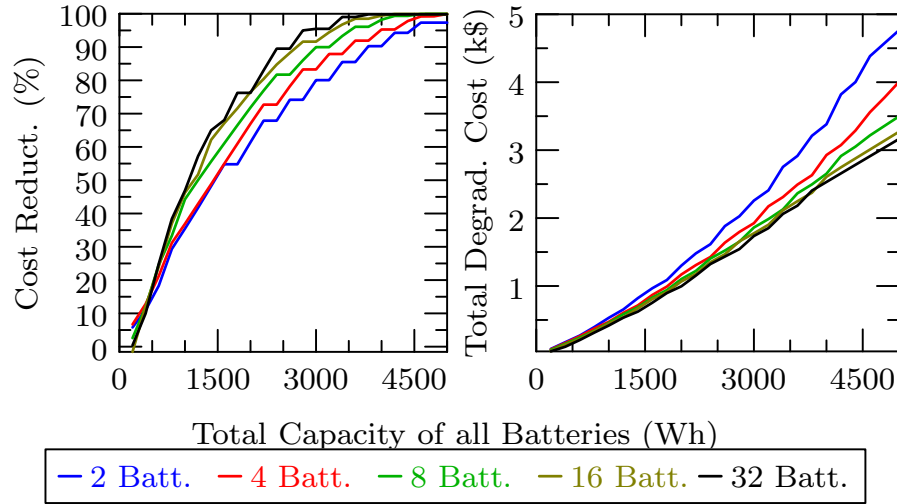
Figure 3.24: Effect of number of batteries on cost reduction and degradation.
