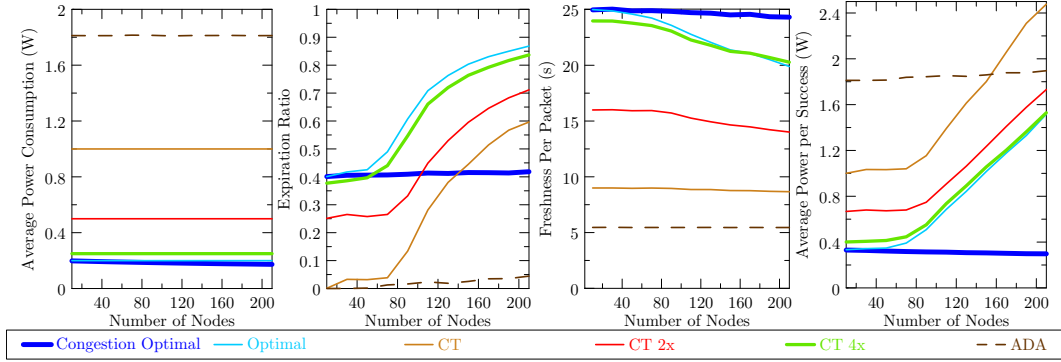
Figure 5.7: 5G network simulation results are provided to study the effect of congestion on the optimal decision. Stream 1: 1s^{-1} rate, information freshness gain function, 1s deadline. Stream 2: 1s^{-1} rate, information freshness gain function, 9s deadline.
