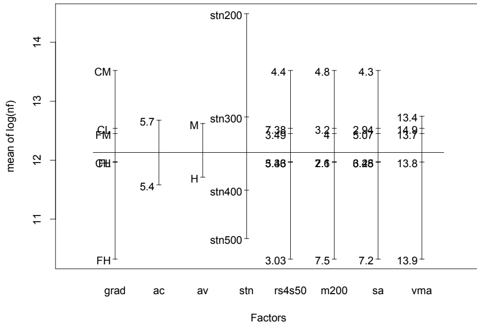
Figure B.4.20. Design plot of lnntf (fatigue test with various gradations at 20°C).
