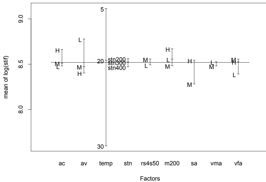
Figure B.4.60. Design plot of lnstif (regression: fine-plus).
