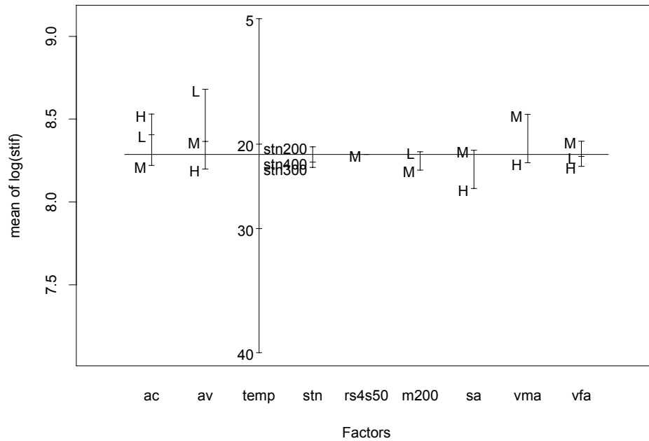
Figure B.4.50. Design plot of \ln(\text{stif}) (regression: fine).
