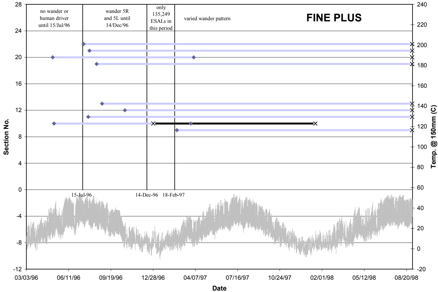
Figure 7.16. The Weibull simulation results and condition survey of fine-plus mixes of the WesTrack project (Note: left ◆ represents the time of SR = 0.8; the right ◆ means the time of SR = 0.6. The left x means the time of 10 % fatigue cracking; the right x is the time of 50 % fatigue cracking.).
