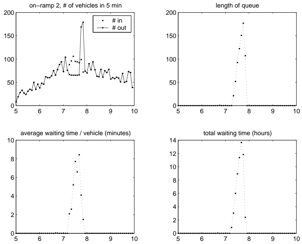
Figure 20: Queue behavior at on-ramp 2 under metering.
