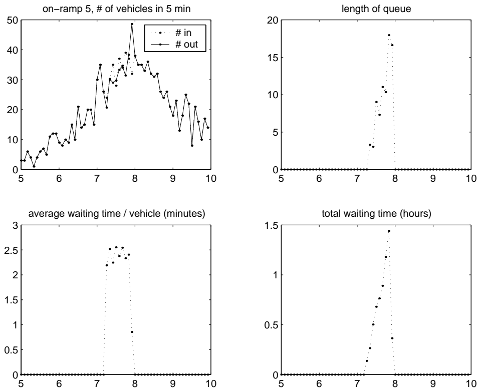
Figure 23: Queue behavior at on-ramp 5 under metering.
