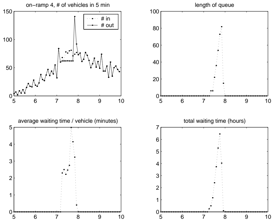
Figure 22: Queue behavior at on-ramp 4 under metering.
