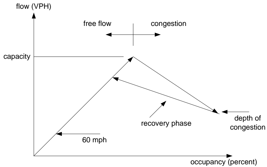
Figure 5: Typical link behavior during a congestion episode. Vehicles travel at 60 mph until flow reaches capacity. Congestion starts. Speed and flow drop, occupancy increases to a maximum value. Demand then drops and speed gradually increases.
