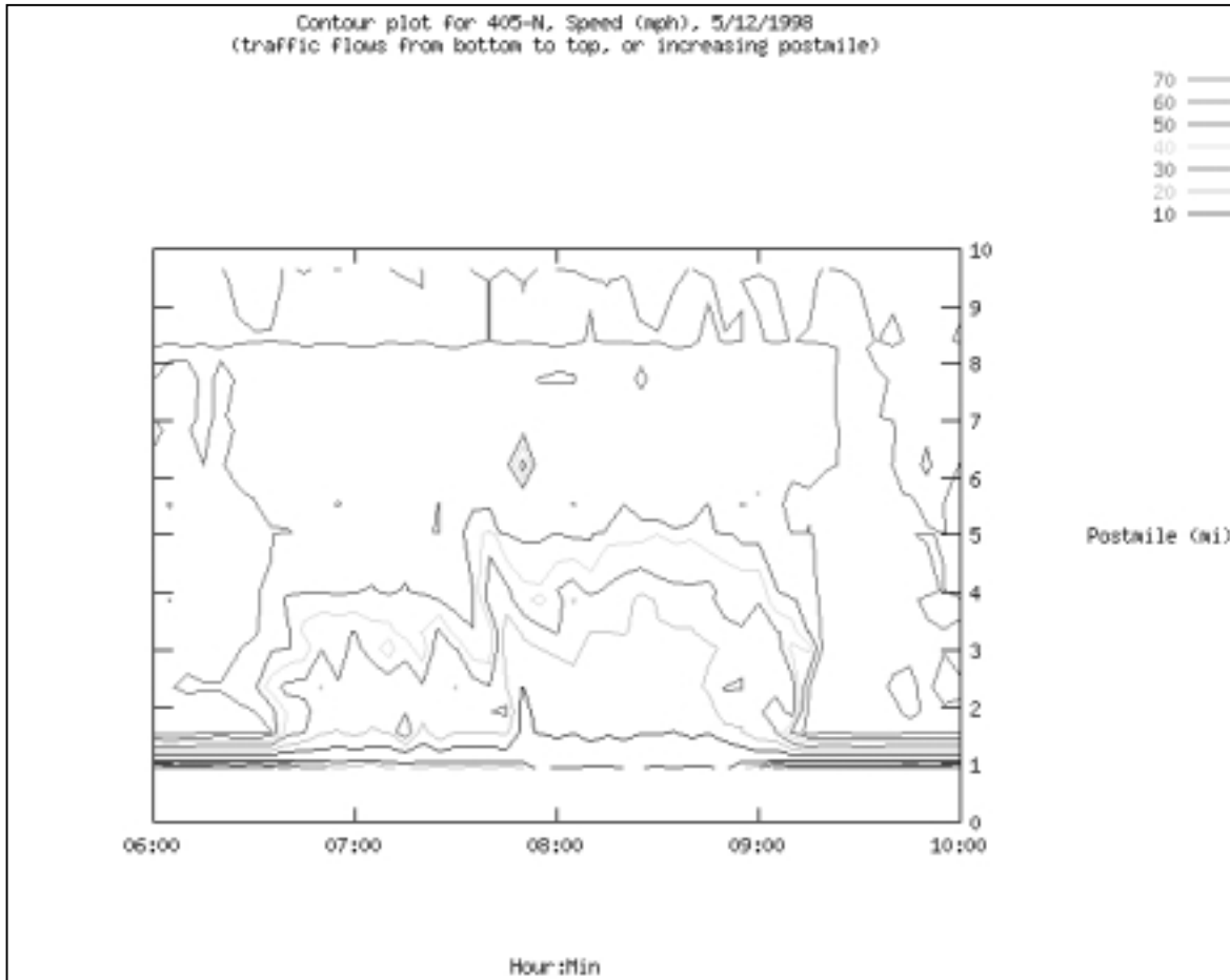
FIGURE 3. Speed Contour Plot along 10 miles of I-405N—6:00 to 10:00 am, 5/12/98
