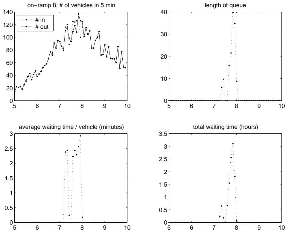
Figure 26: Queue behavior at on-ramp 8 under metering.
