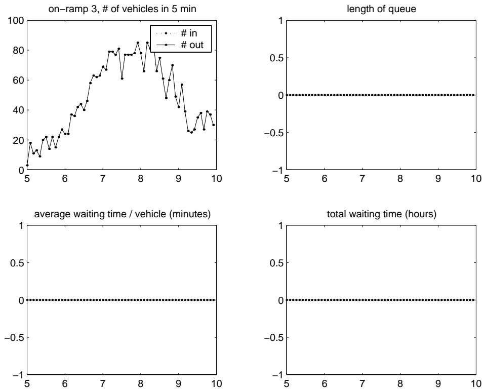
Figure 21: Queue behavior at on-ramp 3 under metering.
