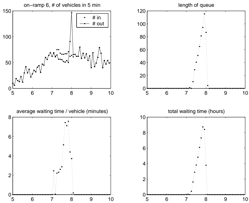
Figure 24: Queue behavior at on-ramp 6 under metering.
