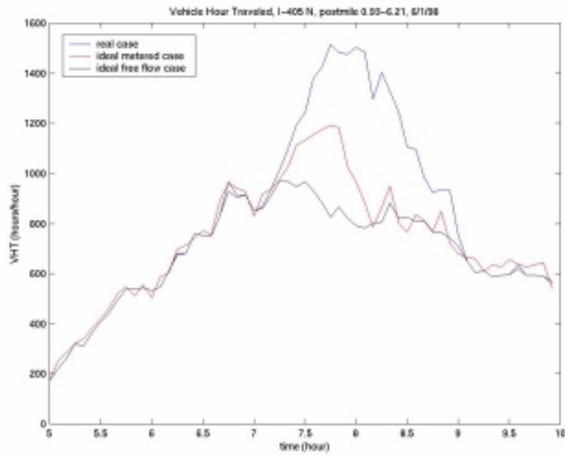
Figure 2: The top graph is the amount of time in VPH actually spent on the freeway section, every 5 minutes. The units are normalized to VPH per hour, so the the total vehicle-hours spent on this section, between 5.00 and 10.00 am is the area under the top graph. The middle graph is the time that would be spent under ideal metering, including time on the ramps. The bottom graph excludes time spent on the ramps, so it is the time that would be spent traveling at 60 mph.
