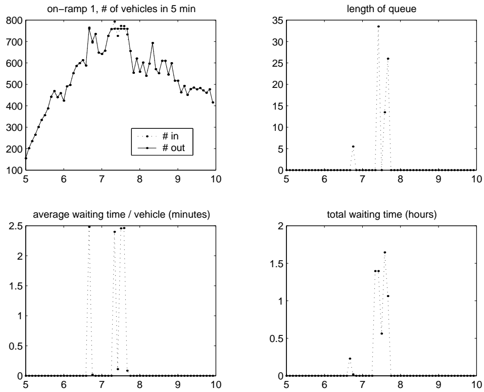
Figure 19: Queue behavior at on-ramp 1 under metering.
