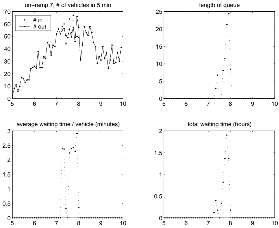
Figure 25: Queue behavior at on-ramp 7 under metering.
