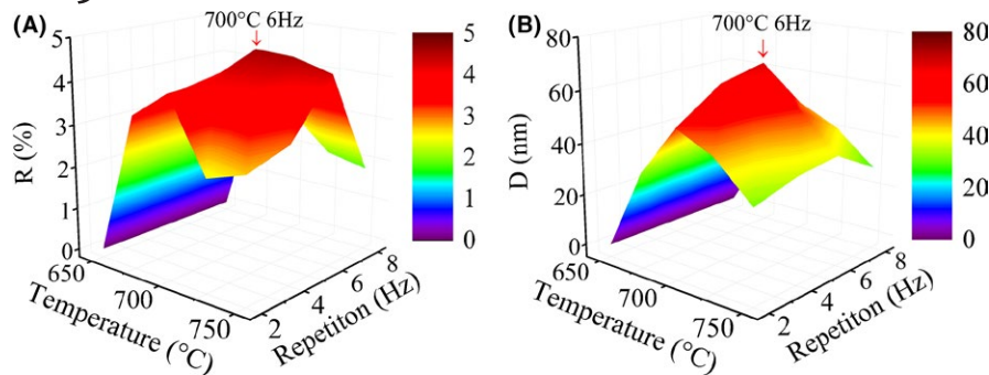
FIGURE 2 Dependence of (A) R ratio and (B) lateral correlation length ( D ) on the substrate temperature and laser repetition rate
