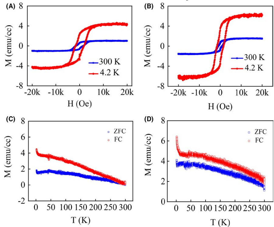
FIGURE 4 The magnetic hysteresis loops of the (111)-oriented BFCO thin films with (A) R = 0\% and (B) R = 4.4\% measured at 300 K and 4.2 K, respectively. Temperature-dependent magnetization of the (111)-oriented BFCO films with (C) R = 0\% and (D) R = 4.4\%
