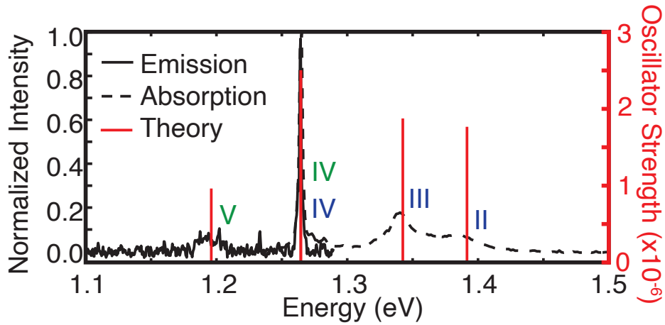
Figure 2.13: Comparison between emission/absorption data and the transition energies and oscillator strength calculated by multireference calculations. Sample used is (thiofan)YbCl(THF).
