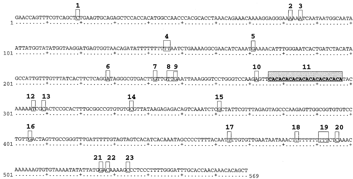
Fig. 1. Full-length consensus sequence of the LPF3 locus in horseshoe crabs (GenBank accession AF020906). The shaded box is the microsatellite repeat region; numbers identify polymorphic sites in the sample of 66 alleles sequenced.
