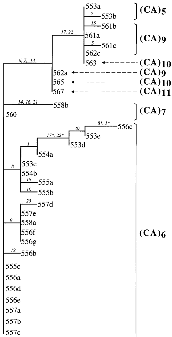
Fig. 2. Allele genealogy for the horseshoe crab LPF3 locus. Shown is the most-parsimonious tree (length = 23 steps, Rescaled Consistency Index = 0.77) reconstructed using polymorphic sites in the microsatellite flanking regions (excluding characters 3, 4, 11, and 19; see Fig. 1). Branch lengths are proportional to numbers of changes; branches of length = zero are collapsed. The number of CA repeats for each allele is indicated on the right. Numbers on branches are particular sequence characters (labeled by number as in Table 1) inferred by the parsimony algorithm to have changed along each branch of the tree. Asterisks indicate character state reversions or parallel changes.
