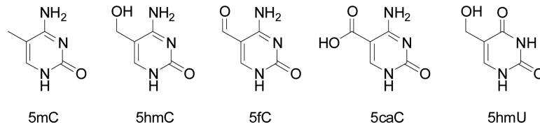
Fig. 1. The chemical structures of 5-methylcytosine and its oxidised derivatives.
