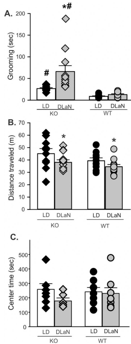
Fig. 7. Repetitive and exploratory behavior are altered by DLaN. Grooming and movement was assessed in a novel arena from mice of each genotype ( Cntnap2 KO, WT) under each lighting condition (LD, DLaN) and the resulting data analyzed with 2-way ANOVA. Histograms show means \pm SEM with the values from individual animals overlaid. Significant ( P < 0.05 ) differences because of treatment are indicated with an asterisk (*) over the treated values while the number sign (#) indicates a genotypic difference. (A) Grooming behavior was significantly increased by genotype ( F_{(1,43)} = 21.986 , P < 0.001 ) and treatment ( F_{(1,43)} = 8.231 , P = 0.007 ). There was a significant interaction between the two factors ( F_{(1,43)} = 5.296 , P = 0.027 ). (B) Novel arena exploration was decreased by the treatment ( F_{(1,43)} = 5.846 , P = 0.020 ) but not genotype ( F_{(1,43)} = 3.603 , P = 0.065 ). (C) The time spent in the center of the open field did not vary with genotype ( F_{(1,29)} = 0.254 , P = 0.619 or
