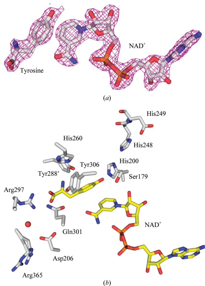
Figure 3 Active site of HinfpDDH . ( a ) Final model of tyrosine and NAD + molecules fitted in 2F_o - F_c electron-density maps prior to model building as output from the last step of XSOLVE (JCSG, unpublished work). The map is contoured at 1\sigma . ( b ) Active site of HinfpDDH showing key active-site residues and the bound tyrosine and NAD + molecules in ball-and-stick representation. C atoms are colored gray for the protein and yellow for the ligands; O, N and phosphate atoms are colored red, blue and orange, respectively.
