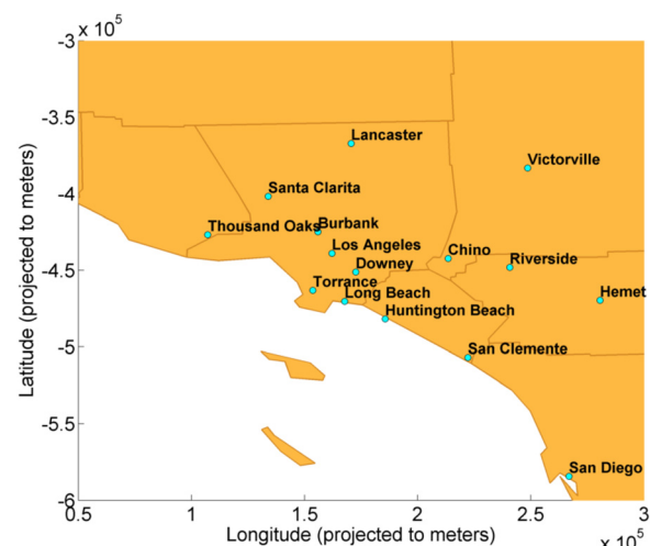
Fig. 6 Detailed view of cities in the SoCAB area of study
