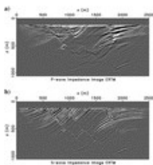
Figure 12. Images obtained via elastic RTM. (a) P-wave impedance perturbation image. (b) S-wave impedance perturbation image.
