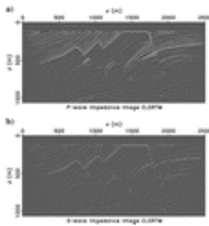
Figure 13. Images obtained via elastic LSRTM. (a) P-wave impedance perturbation image. (b) S-wave impedance perturbation image.
