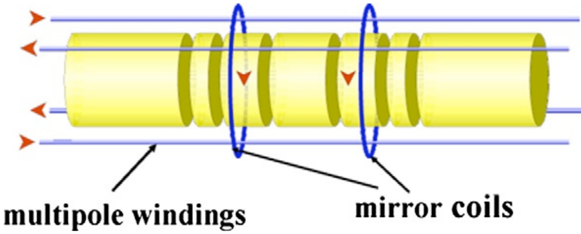
Figure 1: Schematic figure of a Penning-Malmberg trap with additional multipole fields and mirror coils. Such a trap is being considered for anti-hydrogen production experiments
