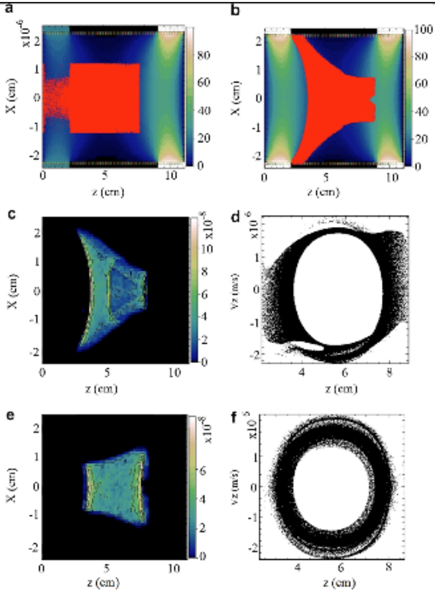
Figure 10: (a) geometry of injection simulations. The color map shows the electrostatic potential and red dots represent the positrons; (b) particles integrated
