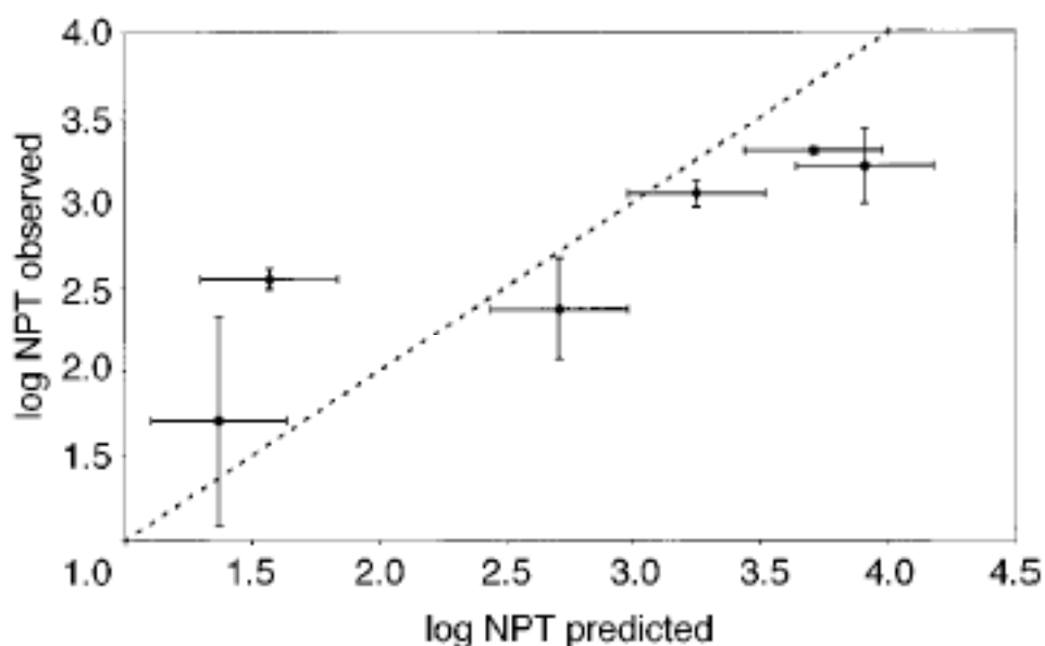
Fig. 1. Observed 40 and estimated values of human nasal pungency threshold log NPT for the terpenes: menthol, linalool, 1,8-cineole, p -cymene, \alpha -terpinene and \Delta -3-carene. The dotted line represents the line of identity; the correlation coefficient is 0.88. Bars indicate standard deviations.
