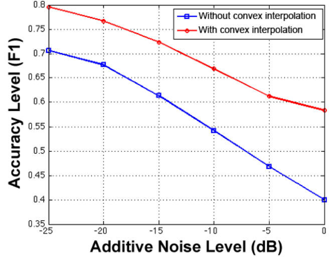
Fig. 10. The average performance of our algorithm with and without convex-hull interpolation vs. various levels of additive noise for 7 Patients (4, 5, 13, 14, 15, 19, and 29).
