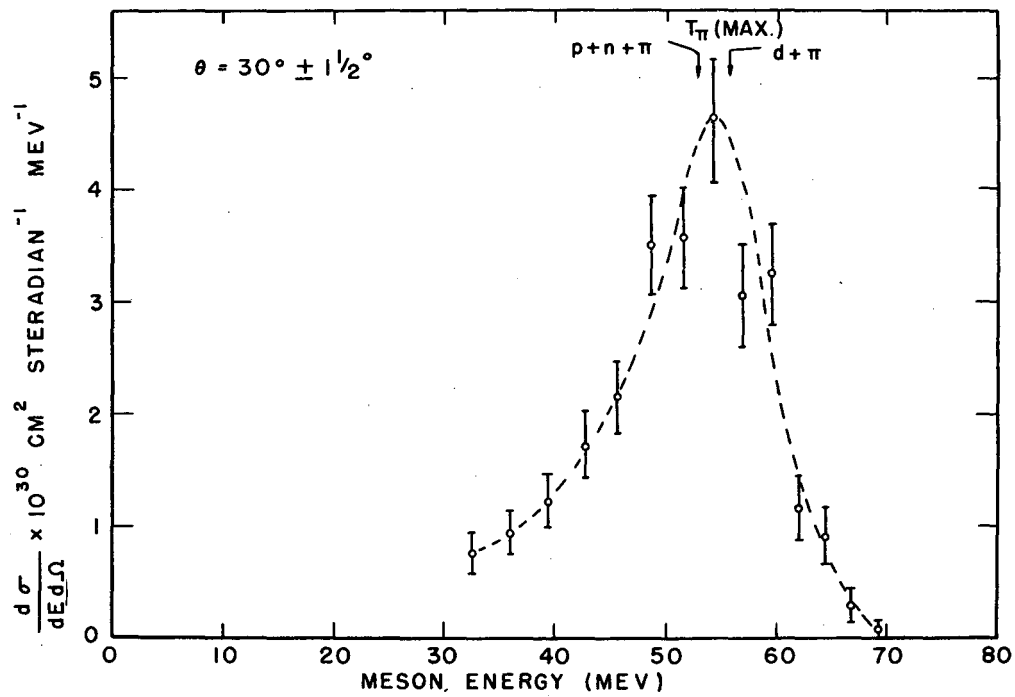
FIG. 15 CROSS SECTION vs. MESON ENERGY AT 30° (POINT SOURCE)
