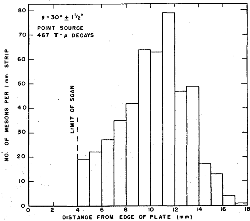
FIG. 14 RANGE DISTRIBUTION OF MESONS (POINT SOURCE RUN)
