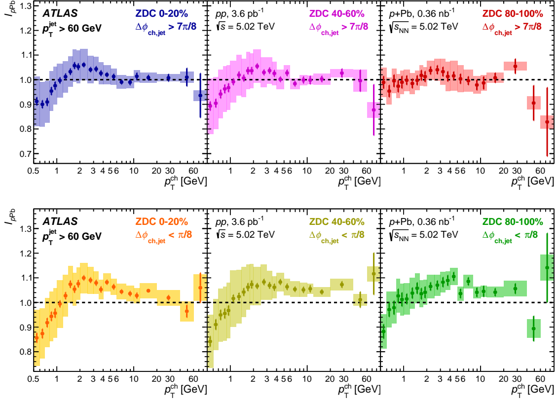
Figure 2: The ratio of per-jet charged-particle yields between p +Pb and pp collisions, I_{pPb} , for hadrons opposite ( \Delta\phi_{\text{ch,jet}} > 7\pi/8 ; top row) and near ( \Delta\phi_{\text{ch,jet}} < \pi/8 ; bottom row) a jet with p_T^{\text{jet}} > 60 GeV. Results are shown for different ZDC-selected p +Pb centralities in each column. Statistical uncertainties are shown as vertical lines and systematic uncertainties as filled boxes.
