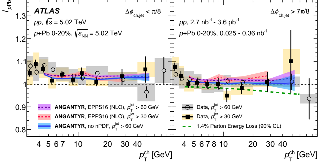
Figure 3: The ratio of per-jet charged-particle yields, I_{pPb} , on the near-side (left) and away-side (right) between p+Pb and pp are plotted for the 0–20% p+Pb ZDC-selected centralities. Particles correlated with a jet above 30 GeV and 60 GeV are shown. Statistical uncertainties are shown as vertical lines and systematic uncertainties as filled boxes. Also shown are calculations from the ANGANTYR generator [57] with two treatments of nuclear-modified parton distribution functions (nPDFs): EPPS16 [58] at next-to-leading order and no nPDF modification, and with a PYTHIA 8-based model for parton energy loss with vacuum fragmentation (see text). ANGANTYR results are only shown for p_T^{\text{ch}} > 4.5 GeV where no UE subtraction is necessary. The colored bands represent statistical uncertainties only.
