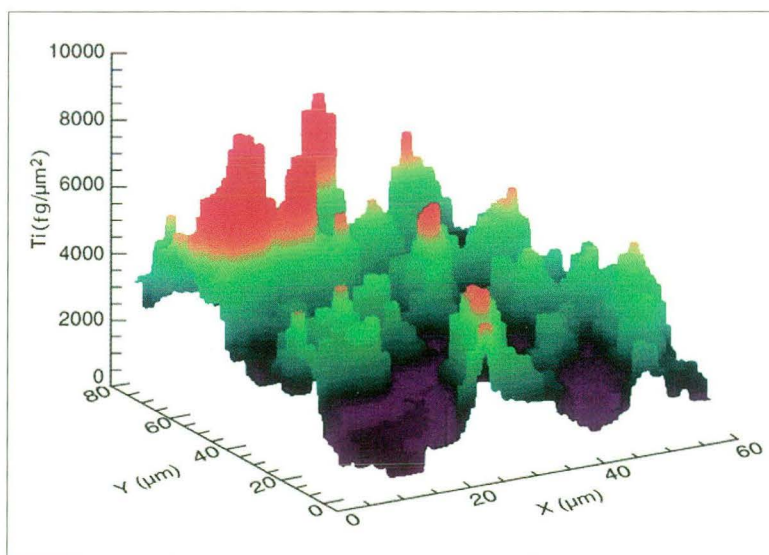
Spatial distribution of titanium in a silicon carbide ceramic from the fluorescence microprobe beamline (Beamline 10.3). Small particles of titanium diboride about 5 \mu\text{m} in diameter can be added to silicon carbide ceramics to improve their mechanical properties, which depend on the uniformity of the distribution of the additive. This scanning x-ray microprobe image indicates that some of the additive has agglomerated into larger particles in this silicon carbide sample.
