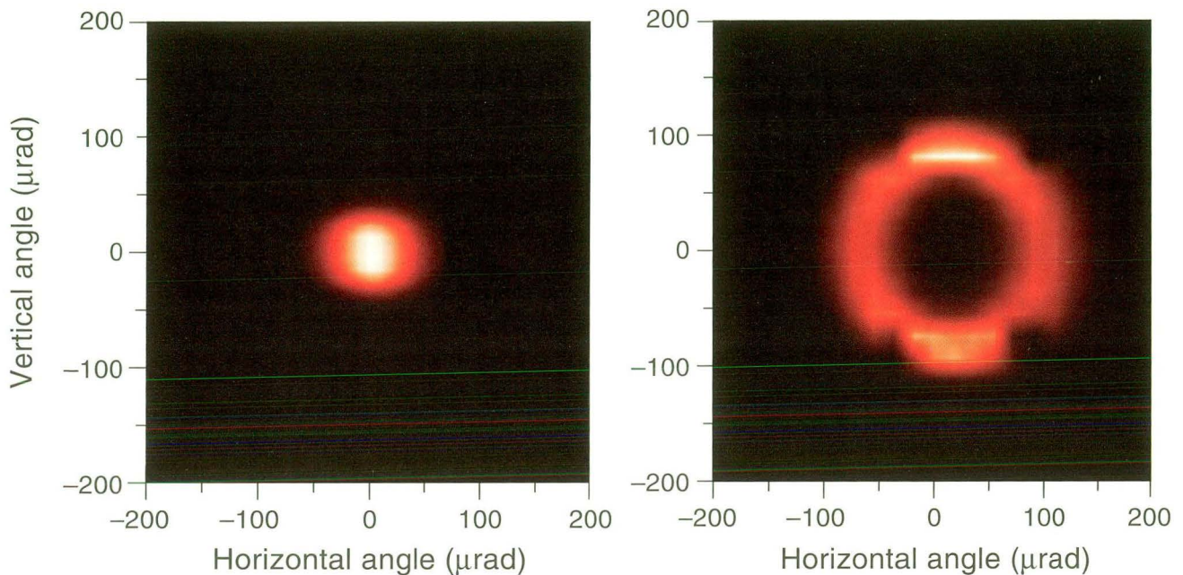
Angular distribution of the US undulator fundamental at K = 0.45 as measured by the transmission grating spectrometer. (Left) If the observation energy coincides with the energy of an odd undulator harmonic (395 eV), one observes a peak in intensity directed along the axis of the electron beam passing through the undulator. (Right) If the observation energy is decreased (374 eV), the emission cannot occur along the axis, but is distributed in a hollow cone of increasing angular width as the energy is decreased. In this image the cone is shadowed by the blades on the beamline's photon-beam-position monitor.
