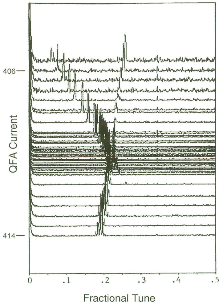
Figure 2. The variation of horizontal and vertical betatron frequencies as a function of the current supplied to the QFA family of focusing quadrupole magnets. The frequencies were measured through Fourier analysis of turn-by-turn data collected by the 96 beam position monitors in the storage ring. The point near the center of the graph where the two traces nearly touch marks a "coupling resonance," a frequency at which energy is exchanged between the horizontal and vertical betatron motions. The distance between the two traces at this frequency provides a measurement of coupling strength. Coupling is of concern to both accelerator physicists and users because it tends to increase the vertical emittance (decreasing brightness).
