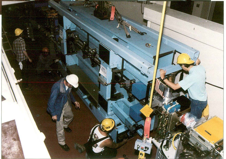
Two US undulators like this one (shown during and after installation) were installed and commissioned in 1993. They are the world's brightest sources of soft x rays.
