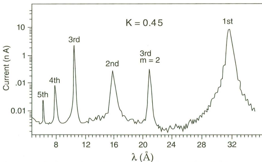
Spectrum of the 5-cm-period undulator taken by the transmission grating spectrometer showing the fundamental and harmonics at a value of K = 0.45 .
