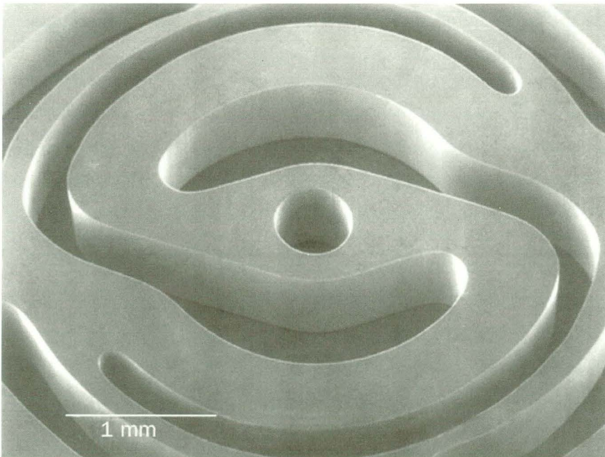
This microstructure, fabricated at the ALS by deep-etch x-ray lithography, could be used in the manufacture of thermal sensing units for automobile engines. The high precision of the lithography process enables complex structures like this to be manufactured with submicron accuracy.
