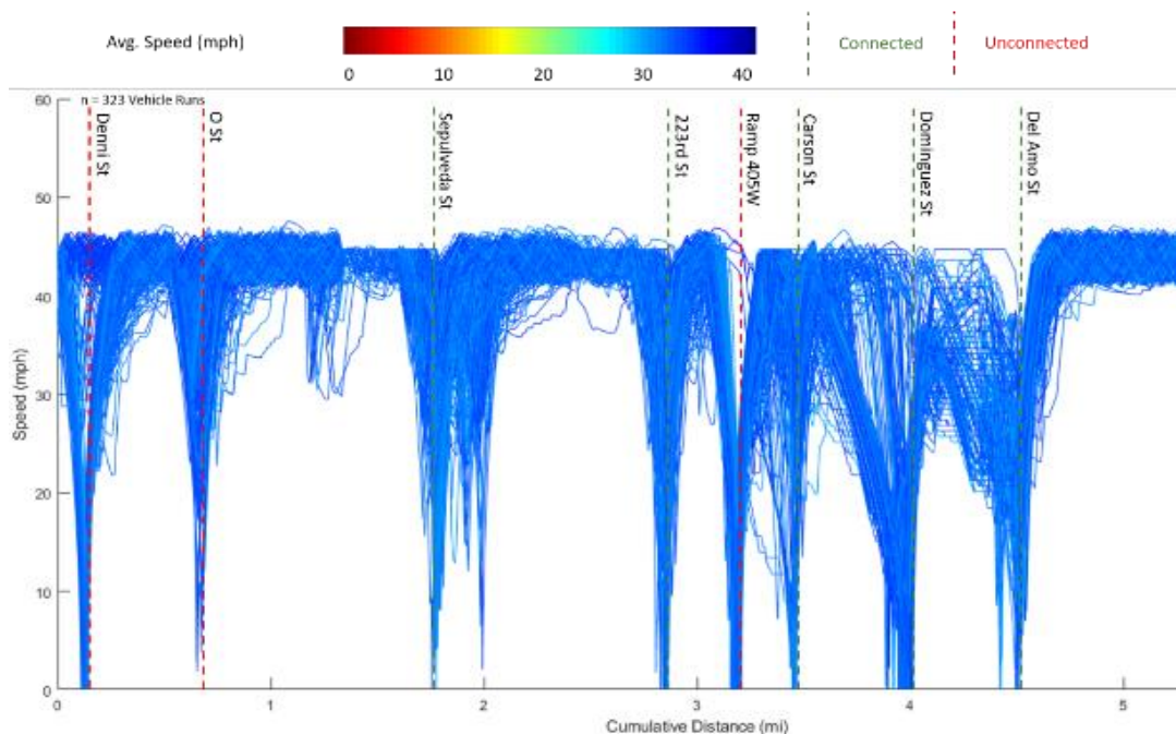
Figure 13. Speed profiles of the connected truck along Alameda St. Northbound
