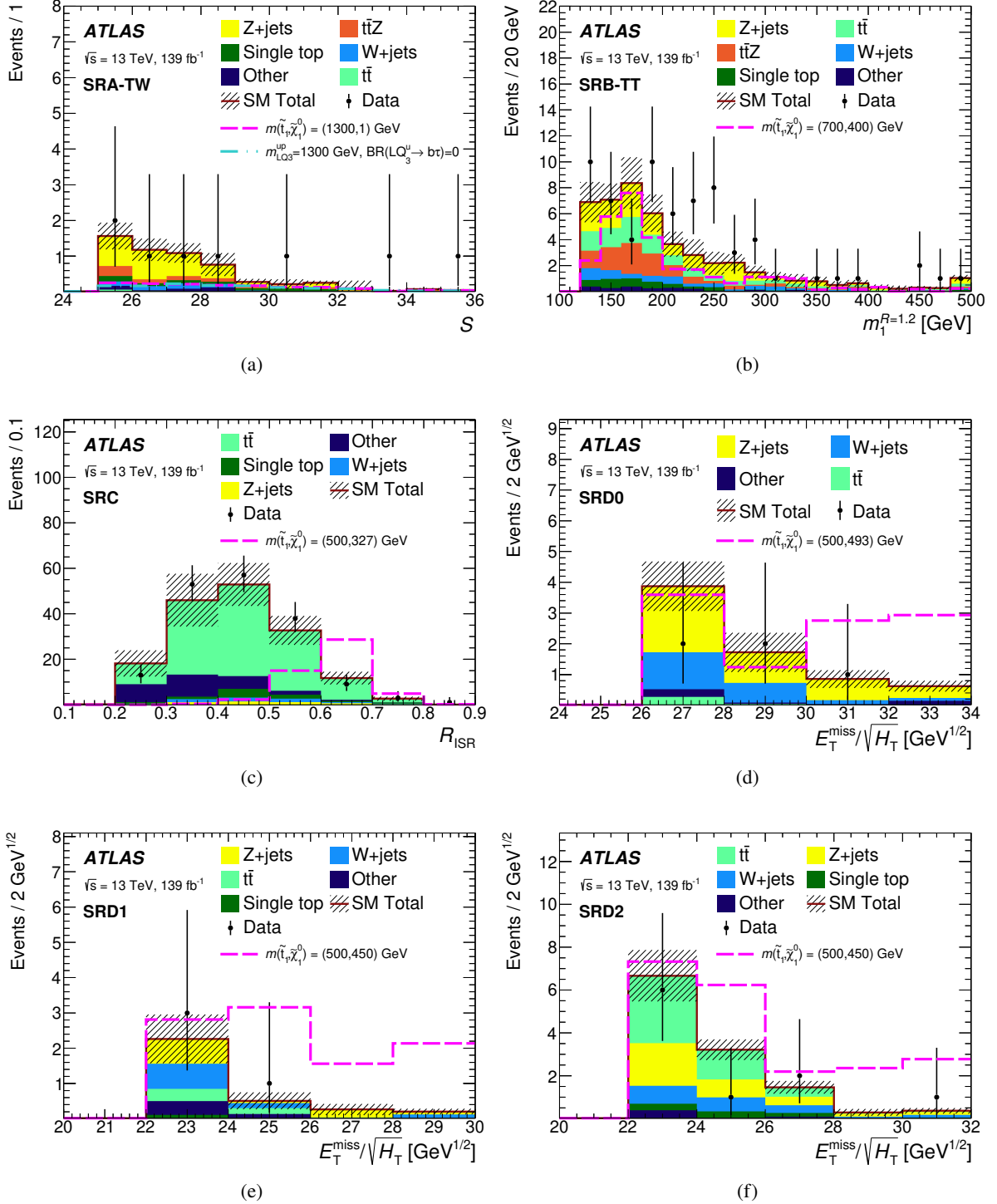
Figure 12: Distributions of (a) \mathcal{S} in SRA-TW, (b) m_1^{R=1.2} in SRB-TT, (c) R_{\text{ISR}} in SRC, and (d–f) E_T^{\text{miss}}/\sqrt{H_T} in SRD0–2 after the SRA–B, SRC and SRD background-only likelihood fits. The stacked histograms show the SM prediction and the hatched uncertainty band around the SM prediction shows the total uncertainty, which includes the MC statistical uncertainties, detector-related systematic uncertainties, and theoretical uncertainties. The data (points) are overlaid. For each variable, the distribution for a representative signal hypothesis is overlaid as a dashed line. The rightmost bin includes overflow events.
