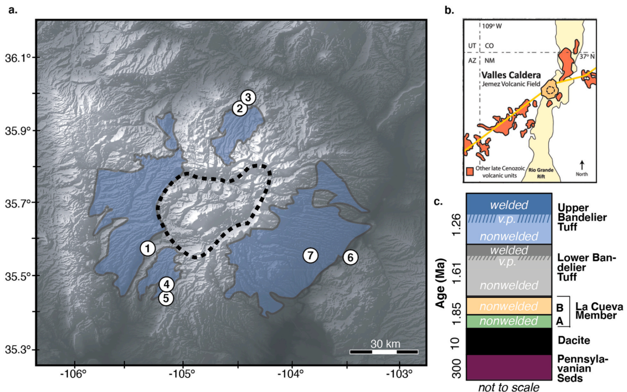
Fig. 1. a) DTM of Valles Caldera with distribution of Banderlier Tuffs (ignimbrites) outlined in blue (after Boro et al., 2021). Dashed heavy line is compound Valles Caldera, the result of two major Banderlier Tuff eruptions. Numbered sites mark field locations: (1) Ponderosa Drive, San Diego Canyon; (2) La Mesita del Cañoncito Seco; (3) Pueblo Mesa, Cañones; (4) Road 10, San Juan Mesa; (5) Upper Paliza Canyon; (6) White Rock Canyon, Cerros del Rio; (7) Frijoles Canyon (see also Table 1 and Supplemental Data Table S1); b) Map showing relationship of Valles Caldera and Jemez (Mountains) Volcanic Field to north-central Rio Grande Rift and line of Cenozoic volcanic fields along Jemez Lineament (orange line, after Goff and Kelley, 2020); c) generalized stratigraphy in western Jemez Mountains (after Gardner et al., 2010 and sources therein); v.p. = vapor-phase altered ignimbrite. (For interpretation of the references to colour in this figure legend, the reader is referred to the web version of this article.)
