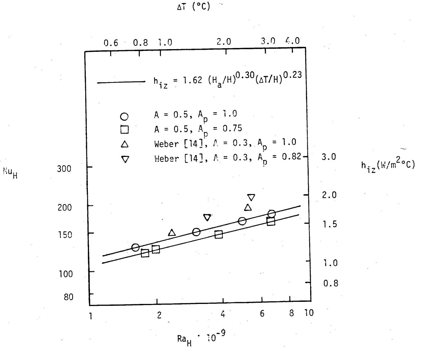
Fig. 10. Interzone Heat Transfer Results and Correlation; Three-Dimensional, Two-Zone Enclosure, Pr = 0.7 (air)
