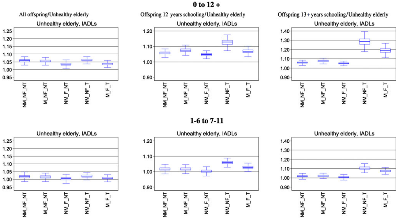
Figure 5. Simulated Generational Support Ratios (GSR)/baseline GSR for instrumental activities of daily living (IADLs).
