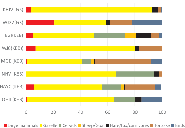
Fig. 4. Relative abundance (%) of prey at Kebaran (KEB) and Geometric Kebaran (GK) sites in the Levant. OHII = Ohalo II (Rabinovich and Nadel, 2005; Simmons and Nadel, 1998); HAYC = Hayonimc Cave C (Stiner, 2005); NHV = Nahal Hadera V (Bar-Oz 2004; Bar-Oz and Dayan 2002); MEG = Meged Rockshelter (Stiner 2005); WJ6 = Wadi Jilat 6 (Garrard and Byrd, 1992); EGI = Ein Gev I (Marom and Bar-Oz, 2008); WJ22 = Wadi Jilat 22 (Martin et al., 2013); KHIV = Kharaneh IV (present study).
