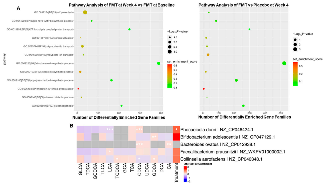
Figure 3. Association between bile acids and bacterial species. (A) Assessment of pathways enriched by FMT relative to baseline (left) and relative to placebo control after 4 weeks of treatment (right). (B) Bacterial species and strains that are correlated with gut bacterial-derived bile acids. * p < 0.2 , ** p < 0.05 , *** p < 0.001 .
