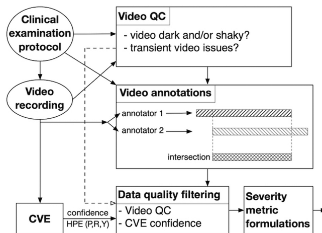
Figure 2. Workflow for CMOR-based video analyses. Data are filtered for quality at the participant level based on the video QC review and at the frame level based on the CVE's confidence in its HPE. Abbreviations: CVE, computer vision engine; HPE, head pose estimates; QC, quality control.
