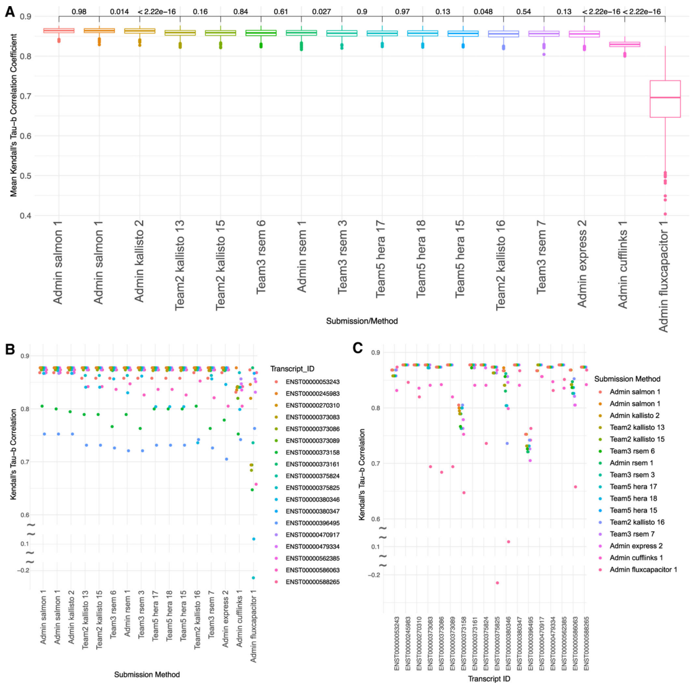
Figure 3. Isoform abundance Kendall Tau- \beta correlation coefficient bootstrap (A–C) Ranking of methods based on their performance in predicting isoform levels as measured by 1,000 bootstrap replicates of the Kendall Tau- \beta score (KTBS) (see STAR methods). The x axis represents the submissions and the y axis the KTBS. Each boxplot represents the 1,000 mean Tau- \beta scores for each bootstrap. Results of the Student’s t test for closely ranked submissions shown between boxplots. Values greater than 0.05 were considered as ties between submissions. (B and C) Kendall’s tau- \beta correlation by transcript and submission method. Plots show Kendall’s tau- \beta correlation coefficient for
