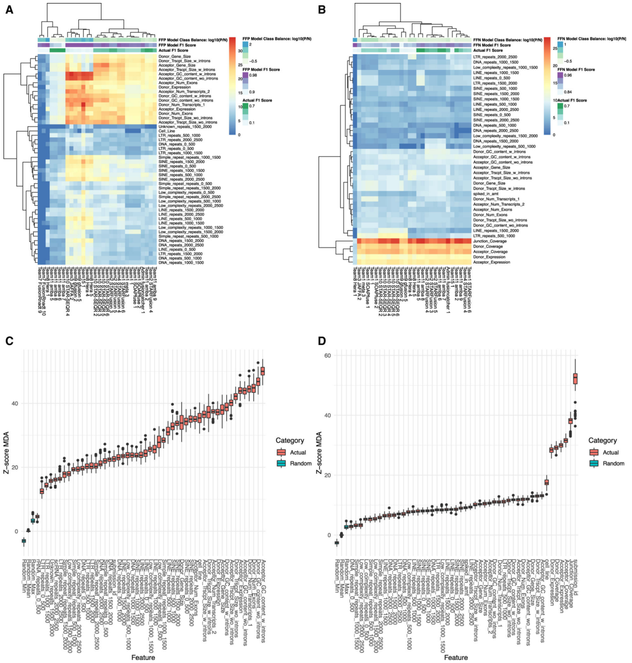
Figure 2. Boruta feature importance analysis across by fusion submissions (A–D) A heatmap showing results from performing the Boruta algorithm on each submission’s false-positive fusion events (A) and false-negative fusion events (B). Each cell in the heatmap represents the Z score mean decrease in accuracy. Higher Z scores are in red and represent more important features. Rows are the fusion submission names and columns are the features. Only features that had a mean value greater than Boruta’s shadow maximum value are shown. Boxplots showing results from performing the Boruta algorithm on all Fusion Detection sub-challenge submissions. (C) is the importance analysis against
