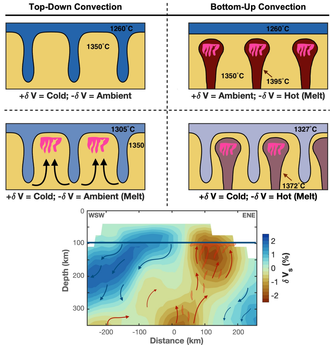
Figure 9. Schematic of possible scenarios for small-scale convective processes compatible with the peak-to-peak anomalies in our body-wave tomographic imaging. Each row either permits or does not allow melt, and each column represents a different set of driving forces for convective processes. In this schematic, the bottom-left panel is our preferred model. Temperatures resulting in our inferred temperature contrast of either \sim 90 K (no melt) or \sim 45 K (melt) are shown; the presence of melt is indicated by orange lenses. The bottom panel shows an annotated cross-section of our preferred S -wave tomographic model, with arrows indicating convective dynamics; the solid line corresponds to the depth to the 1,150 isotherm for 90 Ma seafloor.
