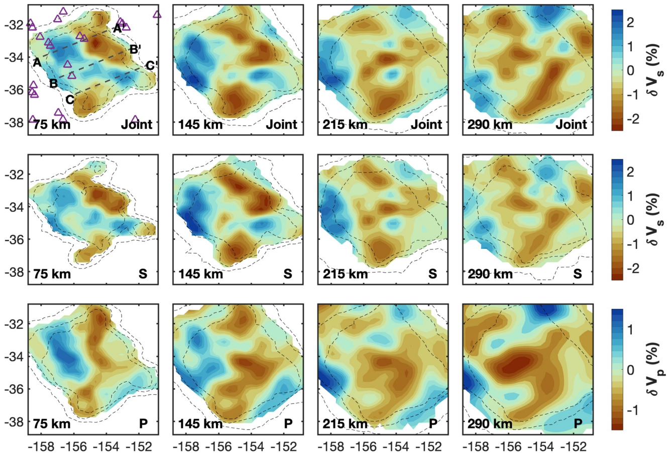
Figure 2. Summary of preferred joint \delta V_s (top row), individual \delta V_s (middle), and \delta V_p (bottom) models at a range of depths. The overlaid dashed lines corresponds to 0.6, 0.4, and 0.2 contours of hit quality; regions with hit quality less than 0.3 are masked out. Each column corresponds to a different depth, which is shown in the bottom-left corner. Purple triangles in the top-left panel correspond to local seamounts from the compilation of Kim and Wessel (2011).
