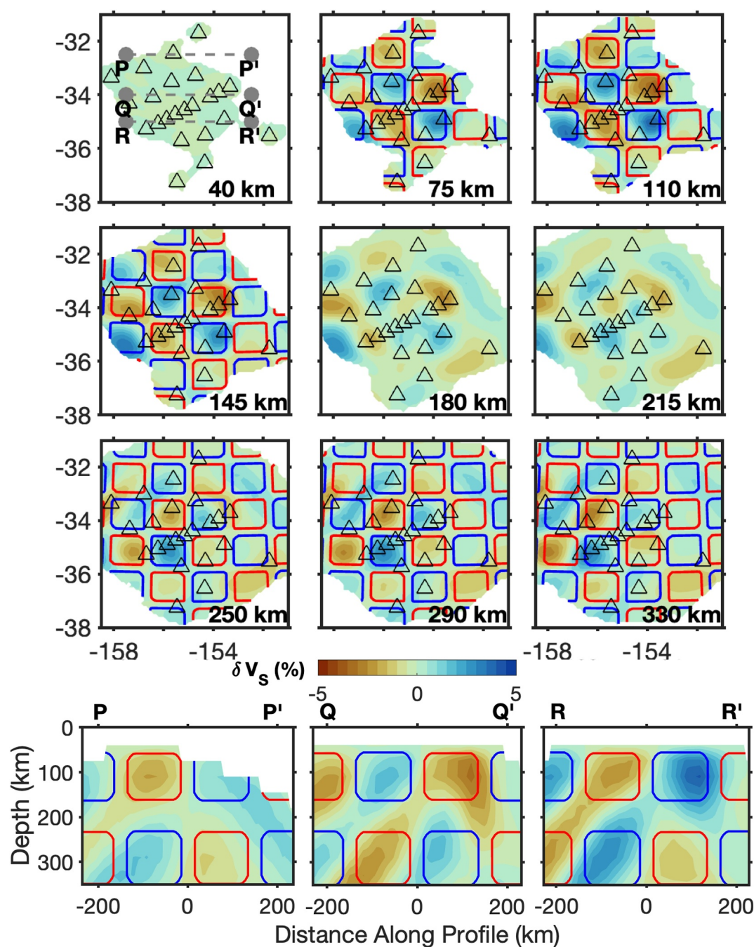
Figure 7. Results of S -wave checkerboard tests. Top three rows; horizontal slices showing the recovery of checkerboard tests at different depths. Bottom row: E-W sections through the output model, with corresponding transects shown in the top-left panel. Only sections of the model with hit quality \geq 0.4 are shown. The locations and shapes of input low and high-velocity checkers of amplitude \pm 5\% are shown with red and blue contours respectively.
