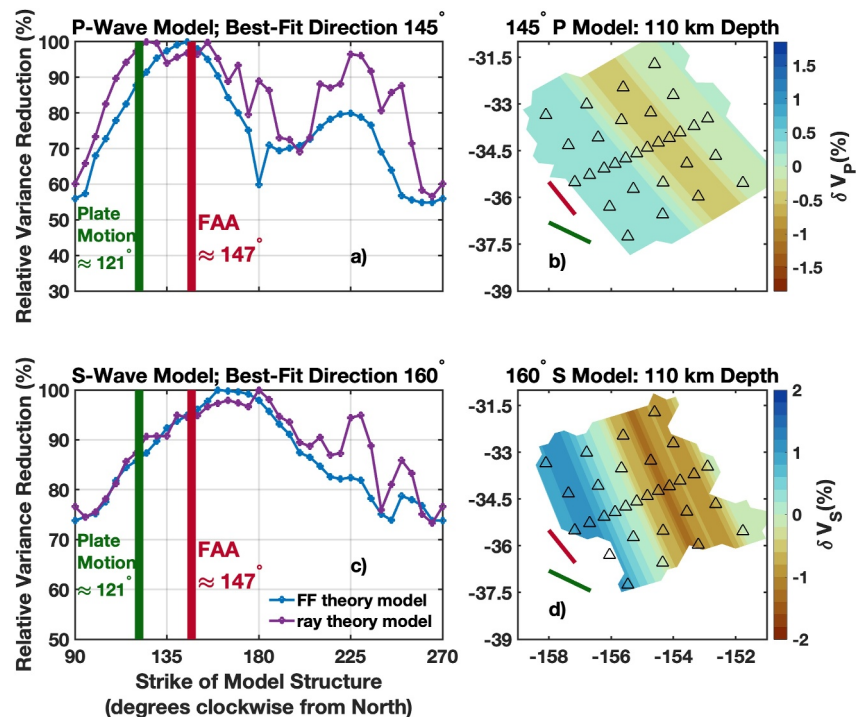
Figure 6. Results of a test to explore the extent to which heterogeneity at a constant orientation can adequately explain our data. (a, c): Variance reduction (Relative to global maximum) as a function of the orientation of model structure, for (a) the P -wave data set and (c) the S -wave data set. Also shown (b, d) are the inverted models that correspond to the best-fitting strike for both the P - and S -wave inversions. Shown as colored lines in panel (d) are the orientations of the free-air gravity anomaly lineations for our study regions and the orientation of absolute plate motion in a no-net rotation reference frame for the ITRF2020 model (Altamimi et al., 2023). Note the consistency between the best-fitting orientation for both P - and S -wave data sets, as well as the consistency in the locations of the low and high-velocity anomalies for the P - and S -wave inverted models.
