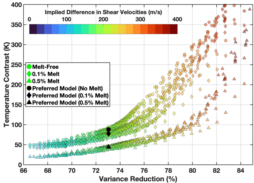
Figure 8. Thermal anomaly implied by the peak-to-peak velocity anomalies in our suite of shear-wave velocity models, spanning a wide range of damping and smoothing parameters. In this context, peak-to-peak velocity anomalies correspond to the difference between the 2.5th and the 97.5th percentile of the velocity anomalies. Circles correspond to a scenario with no melt, diamonds correspond to a scenario with a minimal amount of melt, and triangles correspond to a scenario with a modest amount of melt. Each plotted point corresponds to a different combination of smoothing and damping parameters.
