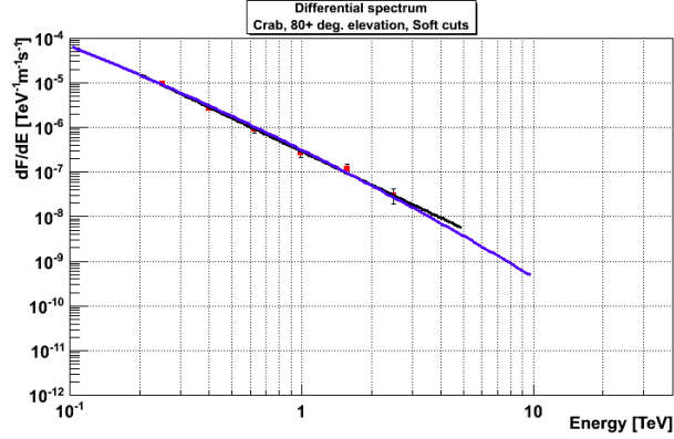
(a) Elevation > 80^\circ
