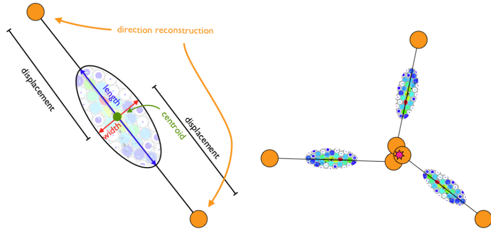
(a) Displacement calculated from (b) Disp method source location reconstruction length/width for a single image.
