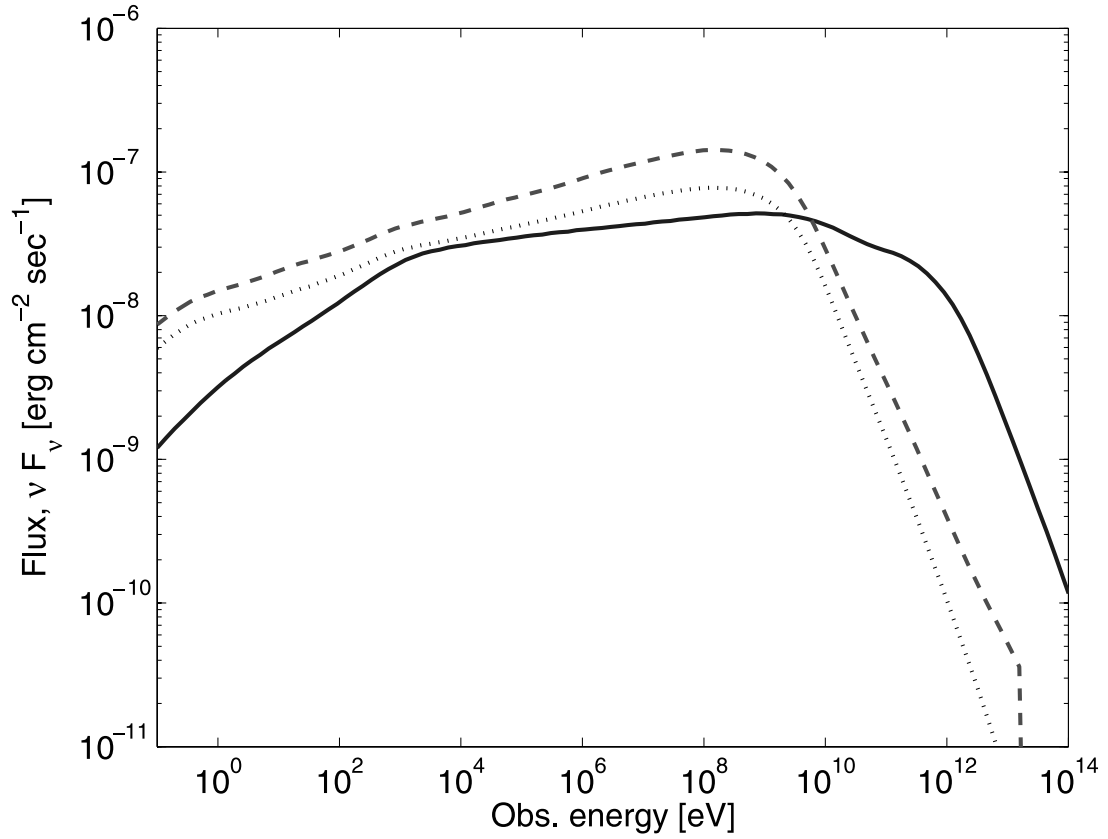
Figure 1.21: Predicted photon spectra during the early afterglow phase for different ISM characteristics. The solid line represents a constant-density ISM ( n = 1 \text{ cm}^{-3} ), while the dashed and dotted lines represent an explosion into a particle wind including and excluding the proton contribution to the flux, respectively. Figure from Pe'er and Waxman (2005).
