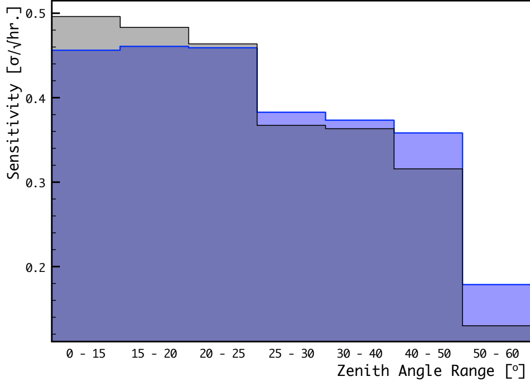
Figure 7.7: The VERITAS sensitivity to a 1% Crab Nebula source over various zenith angle ranges. The blue histogram indicates the disp method sensitivity, and the grey histogram the standard reconstruction method. Both methods are described in Section 8.1.
