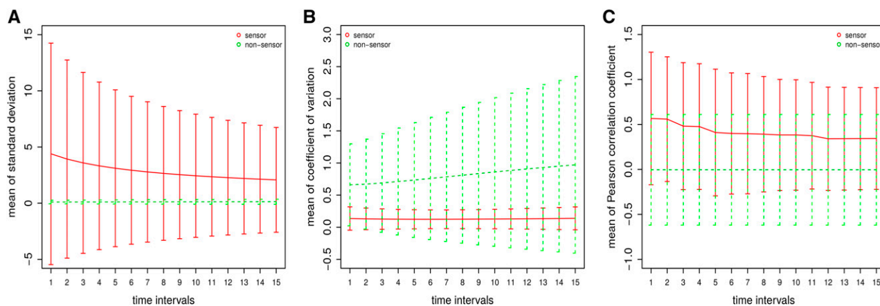
Figure 7. Statistical comparison of the sensors and nonsensors in the kinetic d -time model of plant central carbon metabolism. The x axis represents the investigated time interval, from 1 to 15. The y axis represents values for the three statistics, respectively: A, sd; B, CV; and C, Pearson correlation of sensors and nonsensors. The red line corresponds to the values for the statistics between sensor metabolites, while the green line corresponds to values between nonsensor metabolites. A dot on the line indicates a significant difference at level \alpha = 0.05 between sensor and nonsensors. Bars represent the range \pm 1 sd from the mean value, for five simulations.
