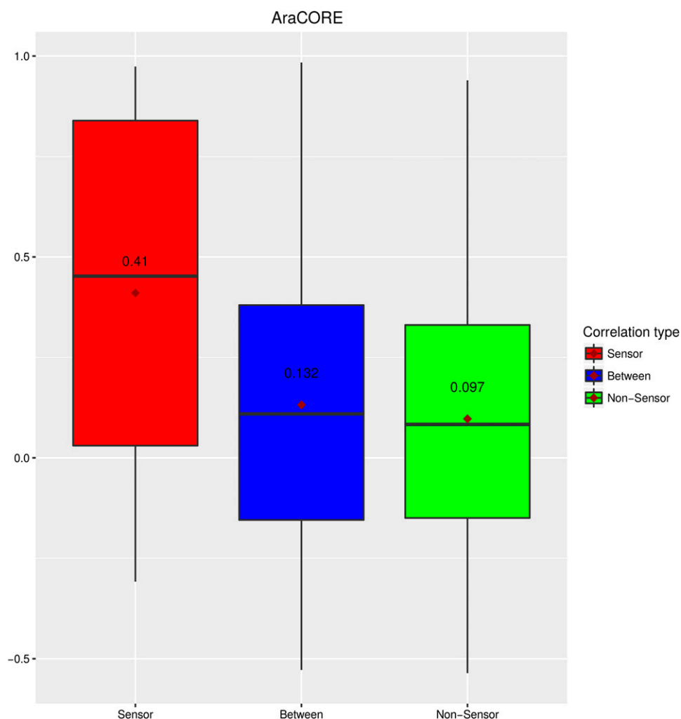
Figure 3. Distribution of correlation values of the AraCORE model. Box plots of the distribution of correlation values between sensors, between sensors and nonsensors, and between nonsensors are colored in red, blue, and green, respectively. The mean value is given above the square symbol, while the median is given by the solid line.
