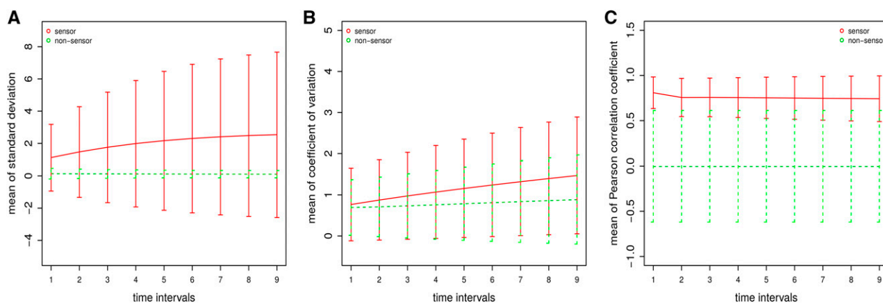
Figure 8. Statistical comparison of the sensors and nonsensors in the kinetic night-time model of plant central carbon metabolism. The x axis represents the investigated time interval, from 1 to 9. The y axis represents values for the three statistics, respectively: A, sd; B, CV; and C, Pearson correlation of sensors and nonsensors. The red line corresponds to the values for the statistics between sensor metabolites, while the green line corresponds to values between nonsensor metabolites. A dot on the line indicates a significant difference at level \alpha = 0.05 between sensor and nonsensors. Bars represent the range \pm 1 sd from the mean value, for five simulations.
