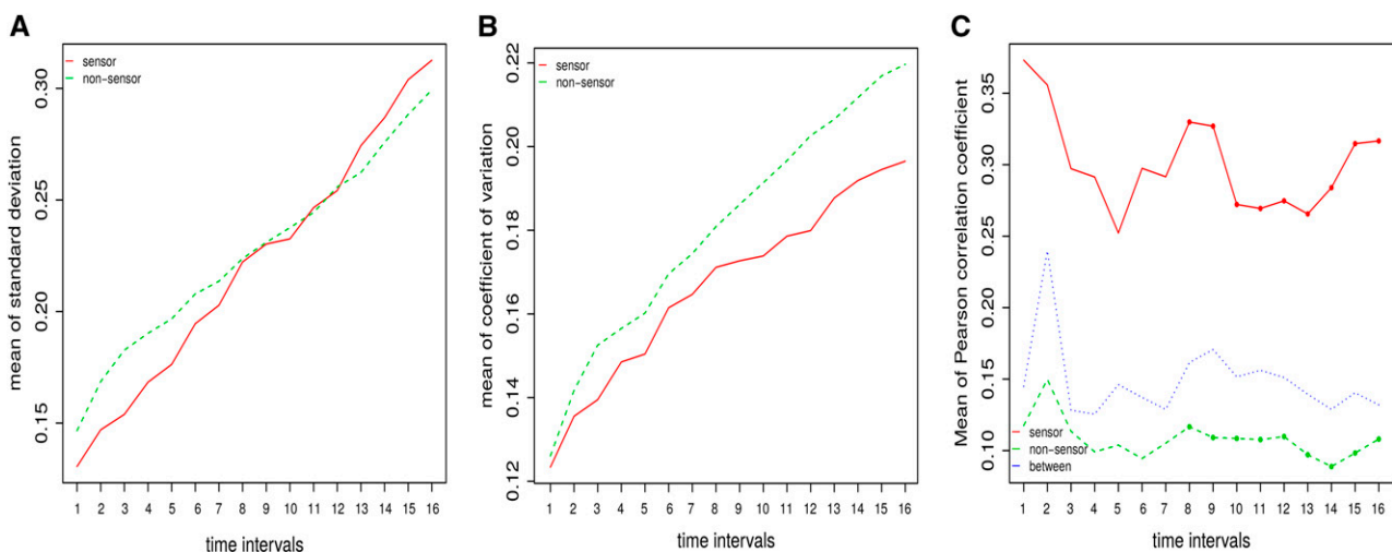
Figure 2. Statistical comparison of sensors and nonsensors in the AraCORE model. The x axis represents the investigated time interval, from 1 to 16. The y axis represents values for the three statistics, respectively: A, SD ; B, CV ; and C, Pearson correlation of sensors and nonsensors. The red line corresponds to the values for the statistics between sensor metabolites, while the green line corresponds to values between nonsensor metabolites. The blue line in C is used for the correlation between sensors and nonsensors. A dot on the line indicates a significant difference at level \alpha = 0.05 between sensor and nonsensors.
