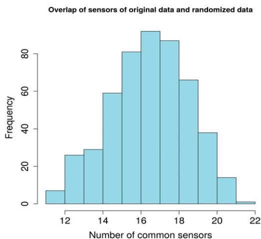
Figure 6. Distribution for the size of the overlap of identified sensors. The distribution is obtained after randomizing the reversibility assignment in the AraCORE model. The x axis displays the number of sensors overlapping with the original analysis. The y axis displays the frequencies of common sensors in 500 shufflings of the reversibility assignment. Originally, 23 sensors were detected.
