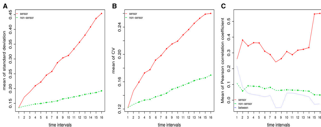
Figure 4. Statistical comparison of sensors and nonsensors in the AraSEED model. The x axis represents the investigated time interval, from 1 to 16. The y axis represents values for the three statistics, respectively: A, SD ; B, CV; and C, Pearson correlation of sensors and nonsensors. The red line corresponds to the values for the statistics between sensor metabolites, while the green line corresponds to values between nonsensor metabolites. The blue line in C is used for the correlation between sensors and nonsensors. A dot on the line indicates a significant difference at level \alpha = 0.05 between sensor and nonsensors.
