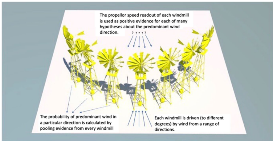
Fig. 2 Windmills used as a probabilistic population code
