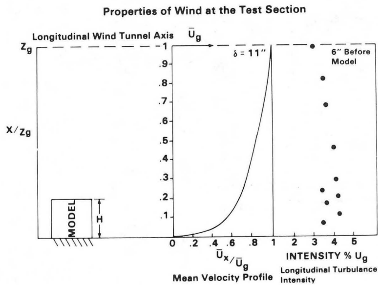
Figure 6. a) NCEL wind-tunnel; b) properties of wind at test section
