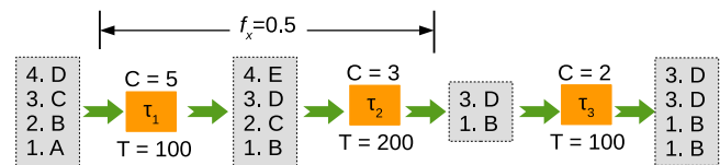
Figure 4: Example of Rule 1 of the pipeline sampling ratio calculation.
