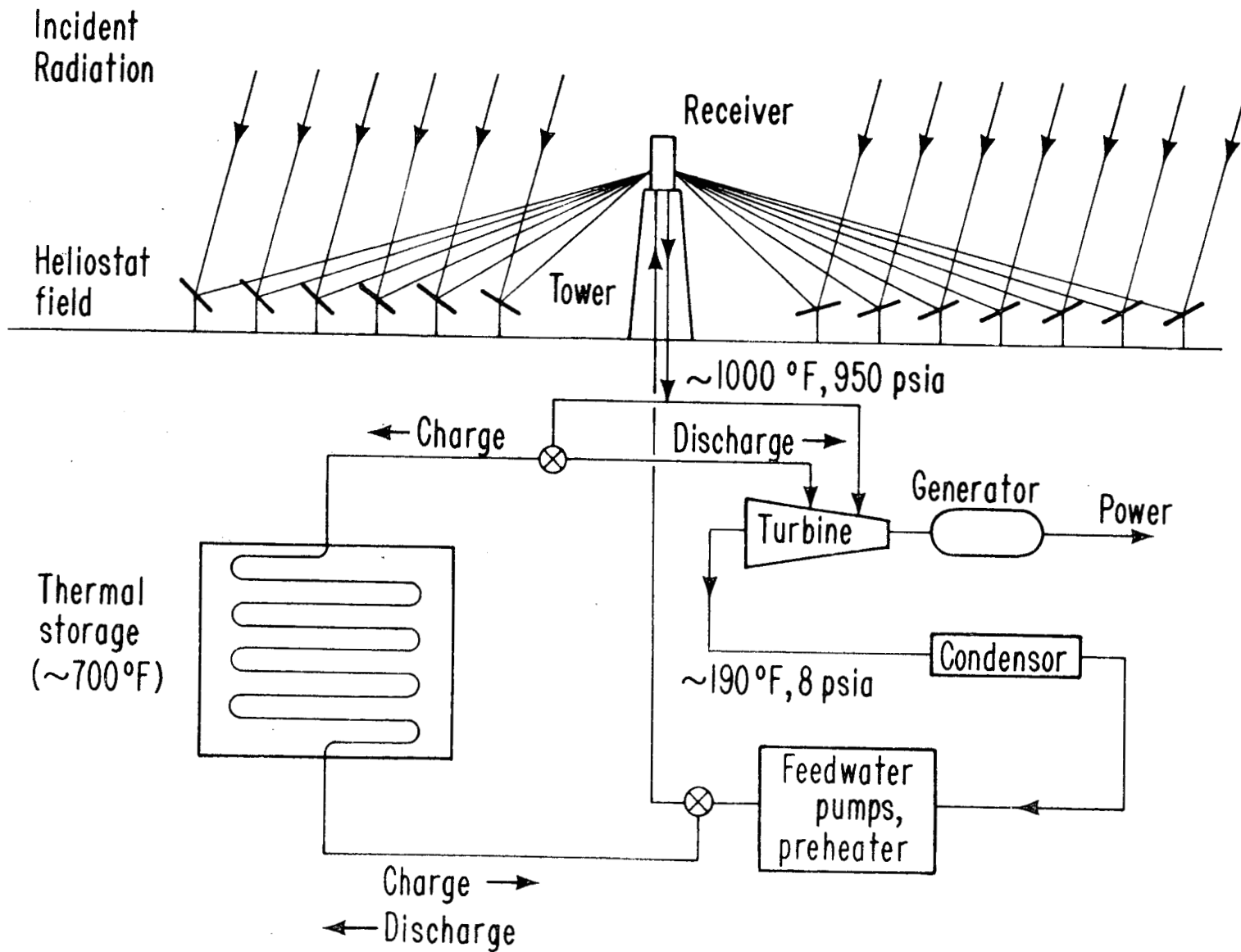
Fig. II-1 Schematic for a Typical Rankine Cycle Central Receiver Power Plant.
