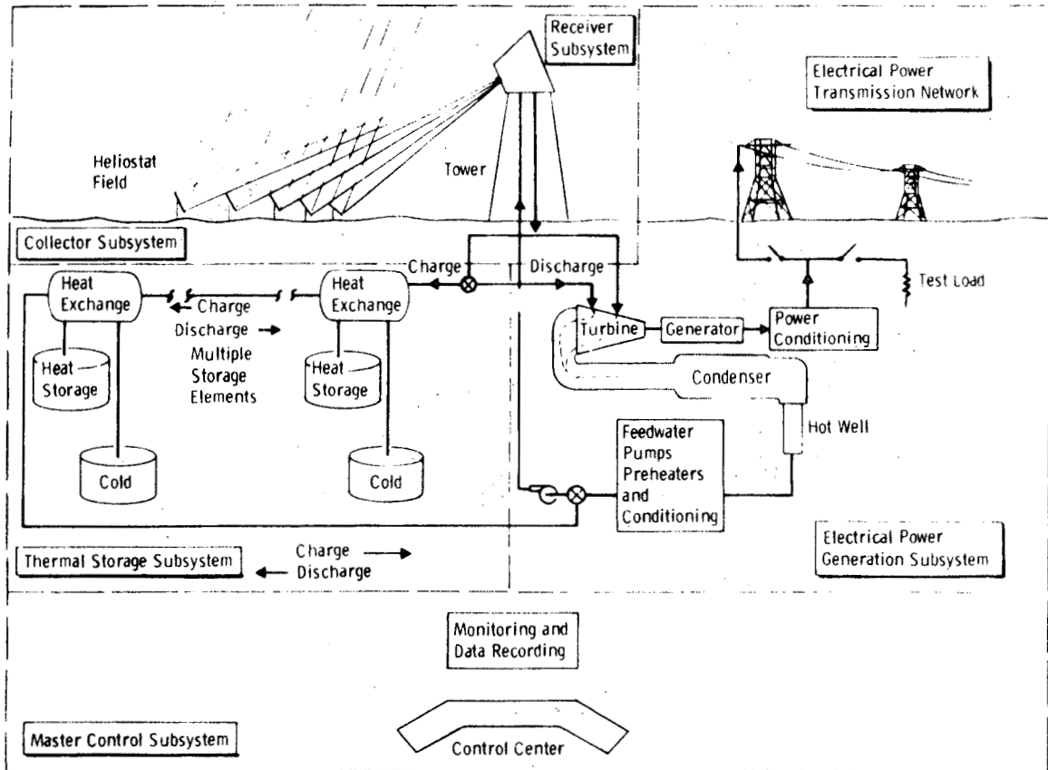
Fig. AII-9 Martin Marietta Preliminary Central Receiver Solar Thermal Power System
