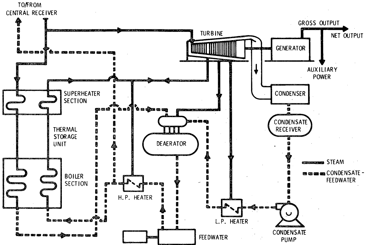
Fig. AII-7 Honeywell Preliminary Central Receiver Solar Thermal Power System
