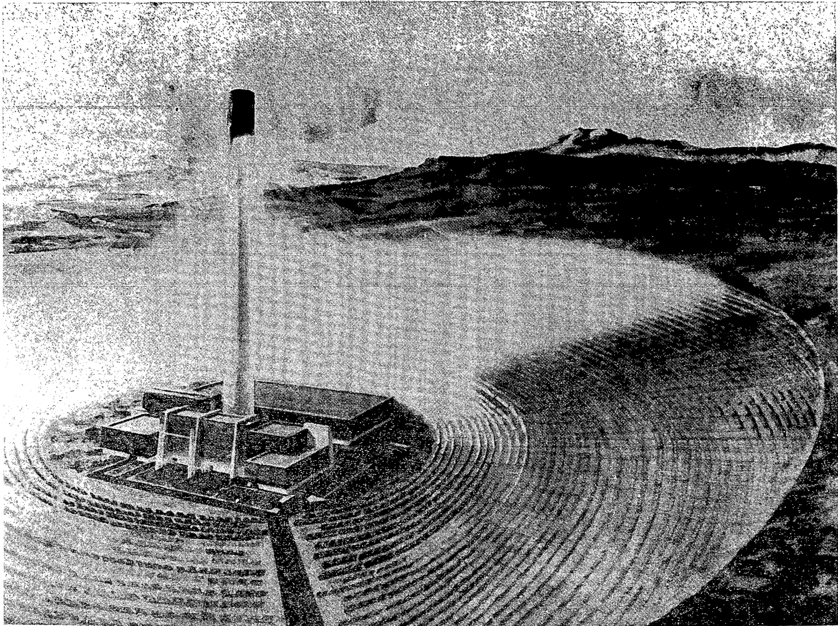
Fig. AII-5 Honeywell 10-MW e Pilot Plant Design. Note that the electrical generation subsystem and thermal storage are located at the base of the tower.
