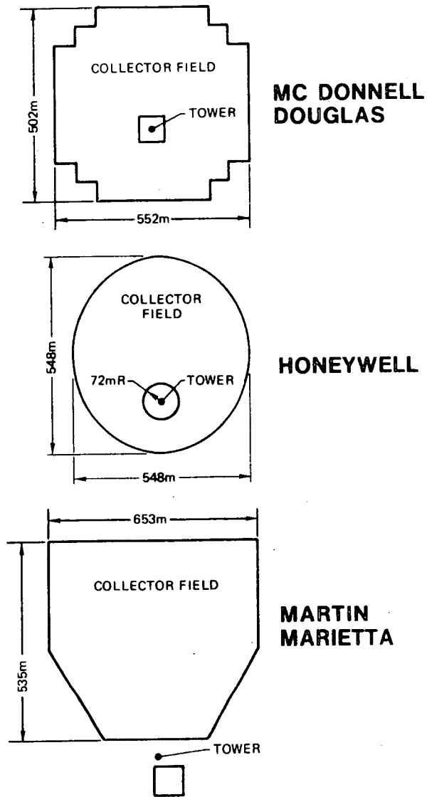
Comparison of the Mirror Field Layouts XBL 774-8285
