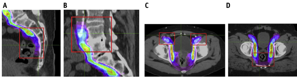
Fig. 2. Count maps showing controversial regions identified.
