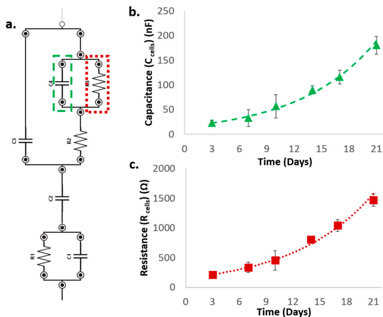
Figure 6. Evolution of the relevant parameters concerning the cell contribution during time ( C_{\text{cells}} , R_{\text{cells}} ). (a): Equivalent circuit with R_{\text{cells}} and C_{\text{cells}} highlighted, (b): Evolution of C_{\text{cells}} during culture, (c): Evolution of R_{\text{cells}} during culture.
