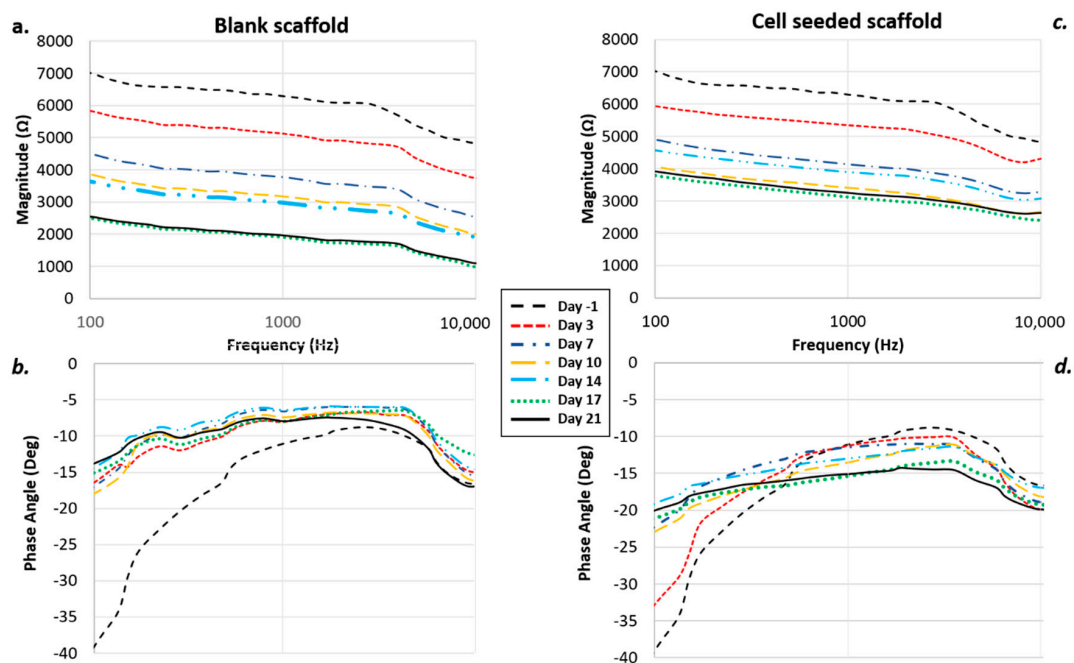
Figure 3. Impedance-based monitoring including controls (a) magnitude and (b) phase angle versus frequency) and seeded scaffolds (c) magnitude and (d) phase angle vs frequency.
