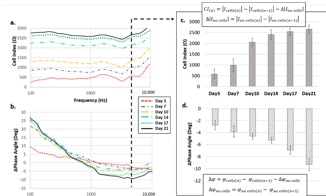
Figure 4. Cell index in terms of (a) magnitude and (b) phase angle contribution to the overall impedance value. Results concerning 4 kHz frequency are specifically highlighted for both (c) magnitude and (d) phase angle.
