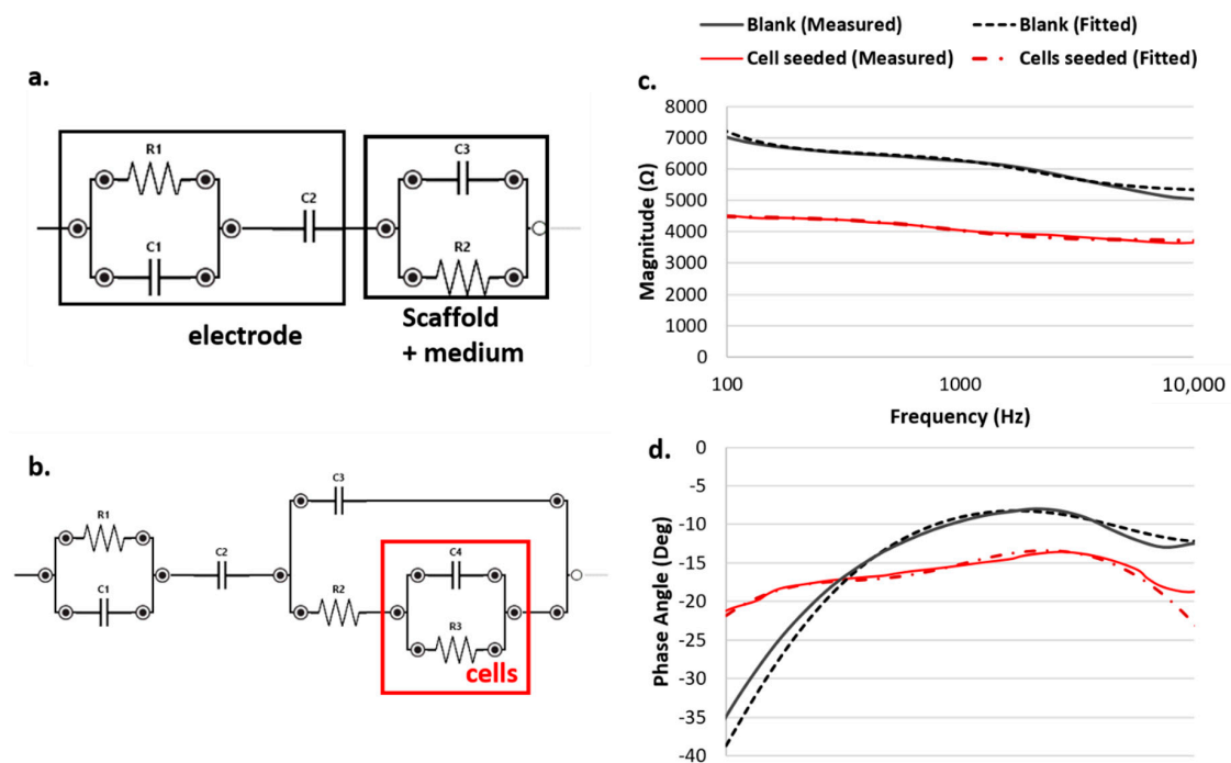
Figure 5. Equivalent circuit modeling the (a) blank and (b) cell seeded conditions: measured and fitted spectra for both the (c) module and (d) phase are reported.
