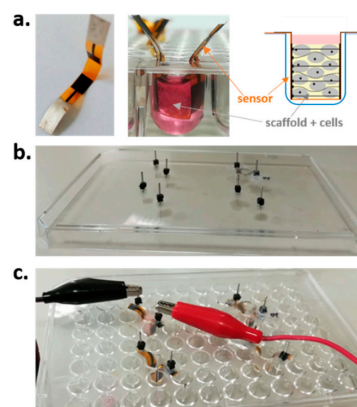
Figure 1. Setup for impedance-based monitoring of human mesenchymal stromal cells (hMSCs) seeded in 3D hybrid hydrogel scaffold: (a) Hybrid hydrogel scaffold and aerosol-jet printed (AJP) sensors, (b) cap for sterile measurements, (c) final measurement setup.
