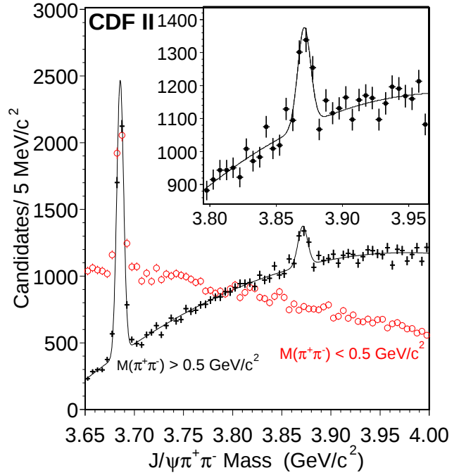
FIG. 2: The mass distributions of J/\psi\pi^+\pi^- candidates with m(\pi^+\pi^-) > 0.5 \text{ GeV}/c^2 (points) and m(\pi^+\pi^-) < 0.5 \text{ GeV}/c^2 (open circles). The curve is a fit with two Gaussians and a quadratic background. The inset shows an enlargement of the high dipion-mass data and fit.
