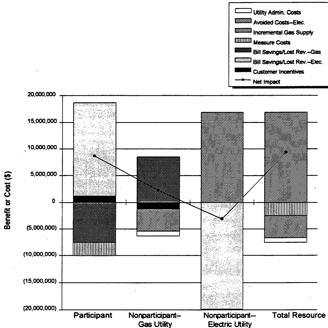
Figure 6-4. Benefit-Cost Tests for an Electric-to-Gas Fuel Substitution Program: Commercial Gas Cooling
