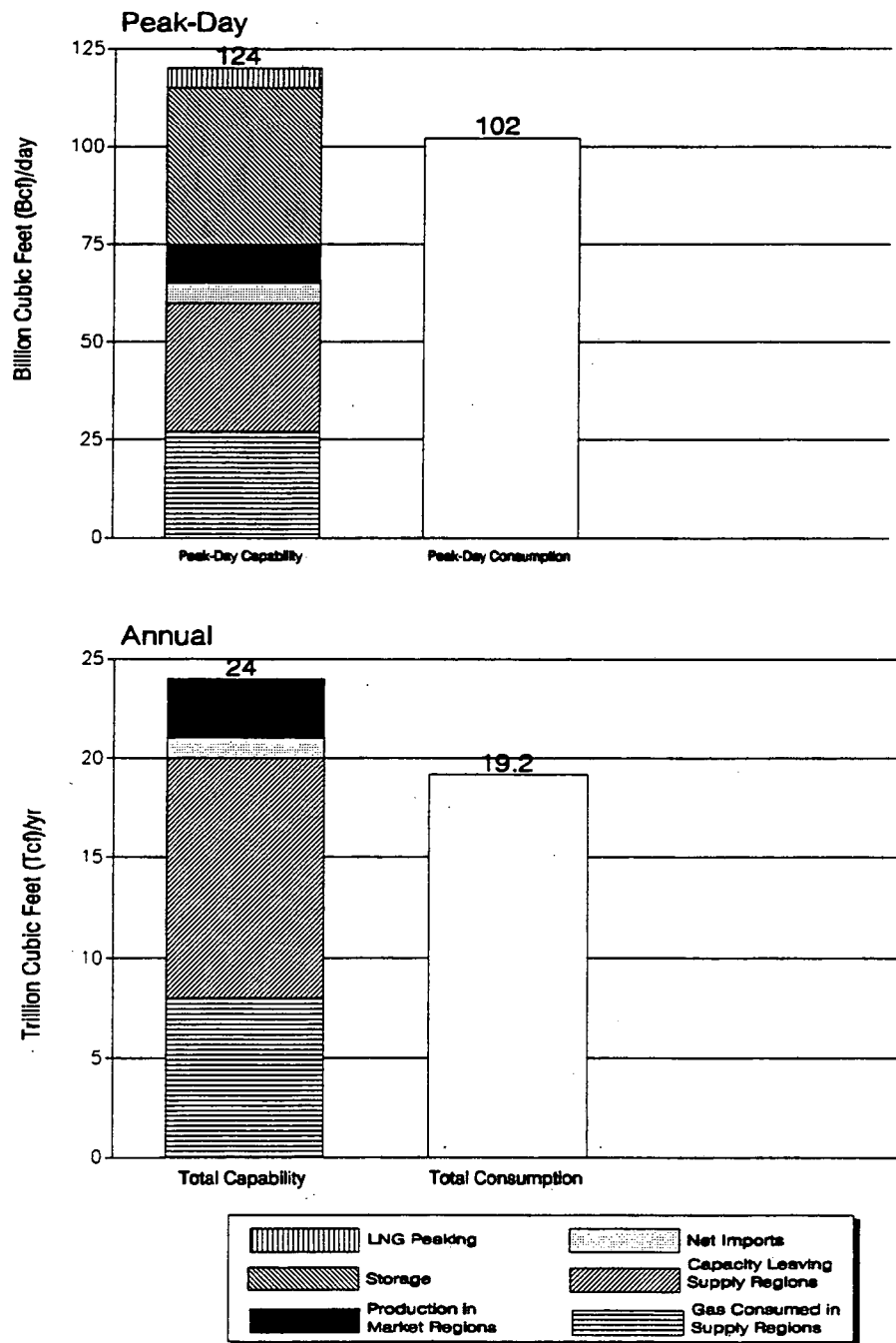
Figure 1-1. U.S. Gas Transmission and Storage System: Peak-Day and Annual Capability (1991)
