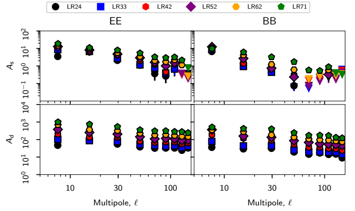
Fig. 8. The amplitudes of EE and BB power spectra for dust and synchrotron emission at 353 and 30 GHz, respectively, shown for each sky region and each multipole bin. The A_s and A_d parameters of our spectral model from Eq. (2) are converted from brightness to thermodynamic (CMB) temperature and expressed in \mu\text{K}^2 . Where the synchrotron amplitude is compatible with zero at the 1\sigma level, we report an upper limit on A_s (68% confidence limit).
