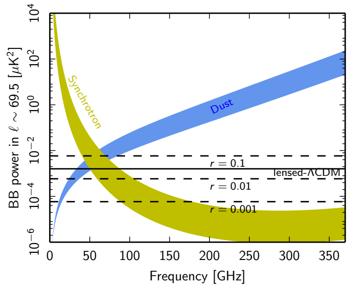
Fig. 12. Dust and synchrotron B -mode power versus frequency for two multipole bins: \ell = 4\text{--}11 (top) and 60\text{--}79 (bottom). The coloured bands show the range of power measured from the smallest (LR24) to the largest (LR71) sky regions in our analysis. The primordial CMB B -mode signal, averaged within the appropriate \ell bin, is plotted with dashed lines for three values of the tensor-to-scalar ratio: r = 0.1 ; 10^{-2} ; and 10^{-3} . The solid line represents the lensing B -mode signal for the Planck 2015 \Lambda CDM model (Planck Collaboration XIII 2016).
