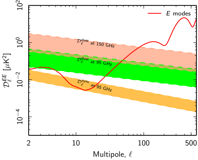
Fig. 10. Dust and synchrotron E -mode power versus multipole. The dust power at 95 and 150 GHz and that of synchrotron at 95 GHz are compared with the CMB E -mode signal (red-line) computed for the Planck 2015 \Lambda CDM model (Planck Collaboration XIII 2016) and a Thompson scattering optical depth \tau = 0.055 from Planck Collaboration Int. XLVI (2016). The coloured bands show the range of power measured from the smallest (LR24) to the largest (LR71) sky regions in our analysis.
