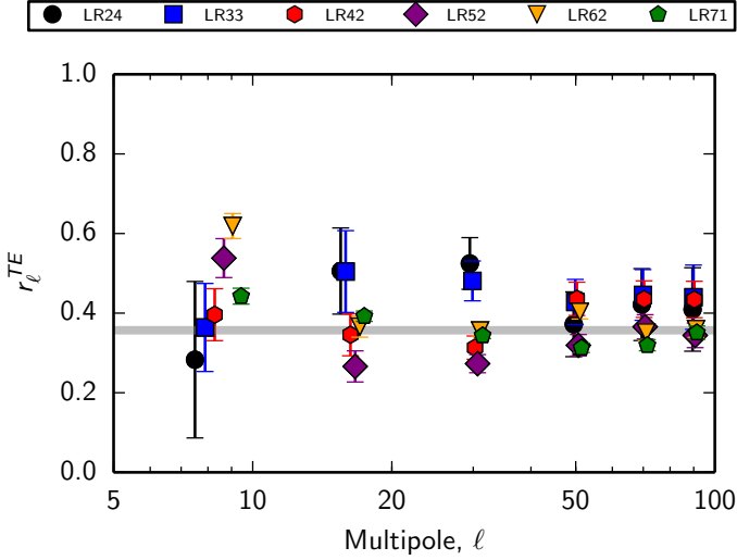
Fig. 4. TE correlation ratio r_{\ell}^{TE} versus multipole. The data points are plotted using distinct symbols and colours (see legend at the top) for each of the six sky regions. The error bars are derived from the E2E simulations.
