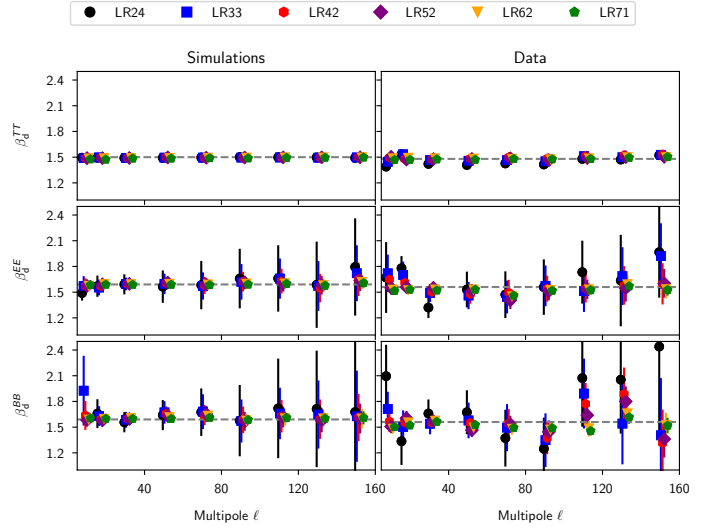
Fig. 14. Comparison of spectral indices of dust polarized emission and total intensity. The spectral indices are derived from the 353-to-217 GHz colour ratio. Plots to the left show the results obtained from our simulated maps, and the ones to the right are from the Planck data. Distinct symbols are used to represent each of the six sky regions, as in Fig. 9. For the simulations, the dashed lines represent the input dust spectral indices ( \beta_d^{TT} = 1.5 , \beta_d^{EE} = \beta_d^{BB} = 1.59 ). For the data, the dashed lines represent the mean measured dust spectral indices ( \beta_d^{TT} = 1.48 , \beta_d^{EE} = \beta_d^{BB} = 1.53 ).
