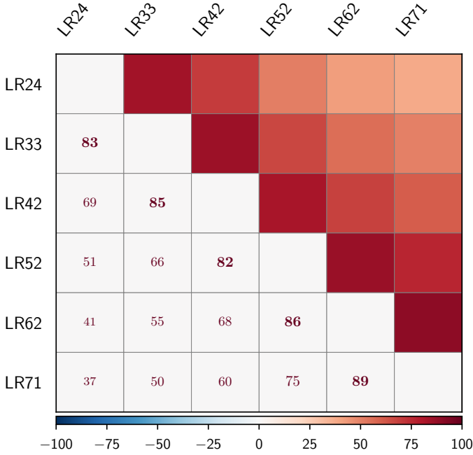
Fig. 17. Cross-correlation factor \mathcal{R}_\ell^{BB} between sky regions, determined from the multi-frequency fits expressed as percentages. As found for the correlation analysis between the 217- and 353-GHz data presented in Appendix B, the results from the multi-frequency fit are correlated between the six nested sky regions.
