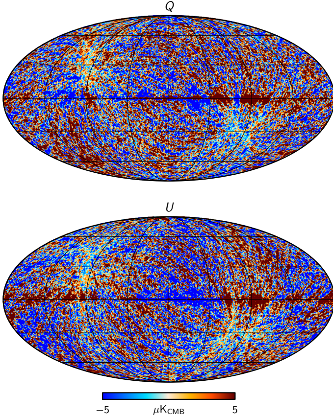
Fig. A.1. Difference between the Stokes Q and U output maps and the sky model inputs at 1^\circ resolution, for one E2E simulation at 353 GHz. Such pairs of difference maps are used to quantify statistical and systematic uncertainties in our analysis of Planck HFI data.
