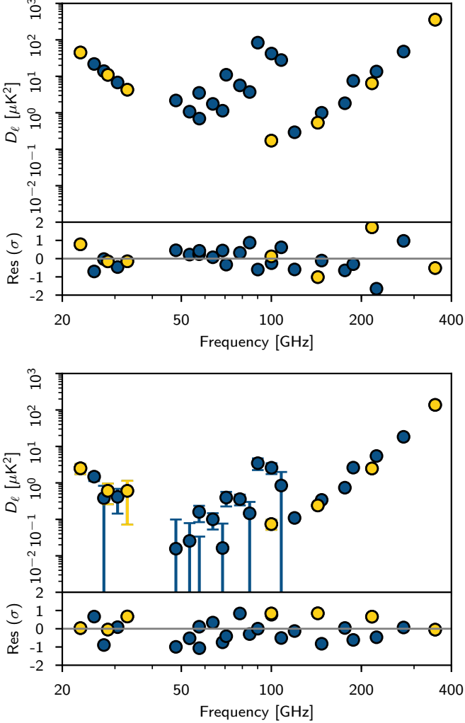
Fig. 6. BB cross-spectra \mathcal{D}_\ell(\nu_1 \times \nu_2) versus the effective frequency \nu_{\text{eff}} = (\nu_1 \times \nu_2)^{0.5} , for the LR62 sky region and two multipole bins: \ell = 4-11 (top plot) and 40-59 (bottom). Yellow and blue colours represent data values from single and inter-frequency cross spectra, respectively. The bottom panel within each plot shows the residuals from the fits normalized to the 1\sigma uncertainty of each data point. Lower frequency data (left) points are dominated by the SED of synchrotron polarized emission, while higher frequency (right) data characterize dust polarized emission, and those at the centre characterize the correlation between the two sources of emission. Differences between the two plots illustrate that both the ratio between synchrotron and dust power and the correlation between these two sources of polarized emission decrease for increasing multipoles.
