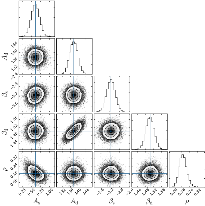
Fig. 7. Posterior distribution for each of the parameters of the spectral model in Eq. (2), as obtained through the MCMC fitting algorithm for BB data points. The MCMC results illustrated here are for the LR62 region and the multipole bin \ell = 40\text{--}59 , one of the two cases shown in Fig. 6. The diagonal shows the probability distribution of each parameter. Median values are A_s = 0.6 \pm 0.1 , A_d = 137 \pm 2 , \beta_s = -3.15 \pm 0.17 , \beta_d = 1.50 \pm 0.02 , and \rho = 0.17 \pm 0.04 .
