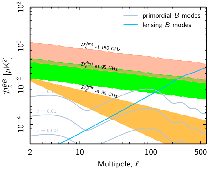
Fig. 11. Dust and synchrotron B -mode power versus multipole. The dust power at 95 and 150 GHz, and that of synchrotron at 95 GHz are compared with CMB B modes from primordial gravitational waves (grey lines) for three values of the tensor-to-scalar ratio, r = 0.1 , 10^{-2} , and 10^{-3} , and from lensing (blue line) for the Planck 2015 \Lambda CDM model (Planck Collaboration XIII 2016). The coloured bands show the range of power measured from the smallest (LR24) to the largest (LR71) sky regions in our analysis.
