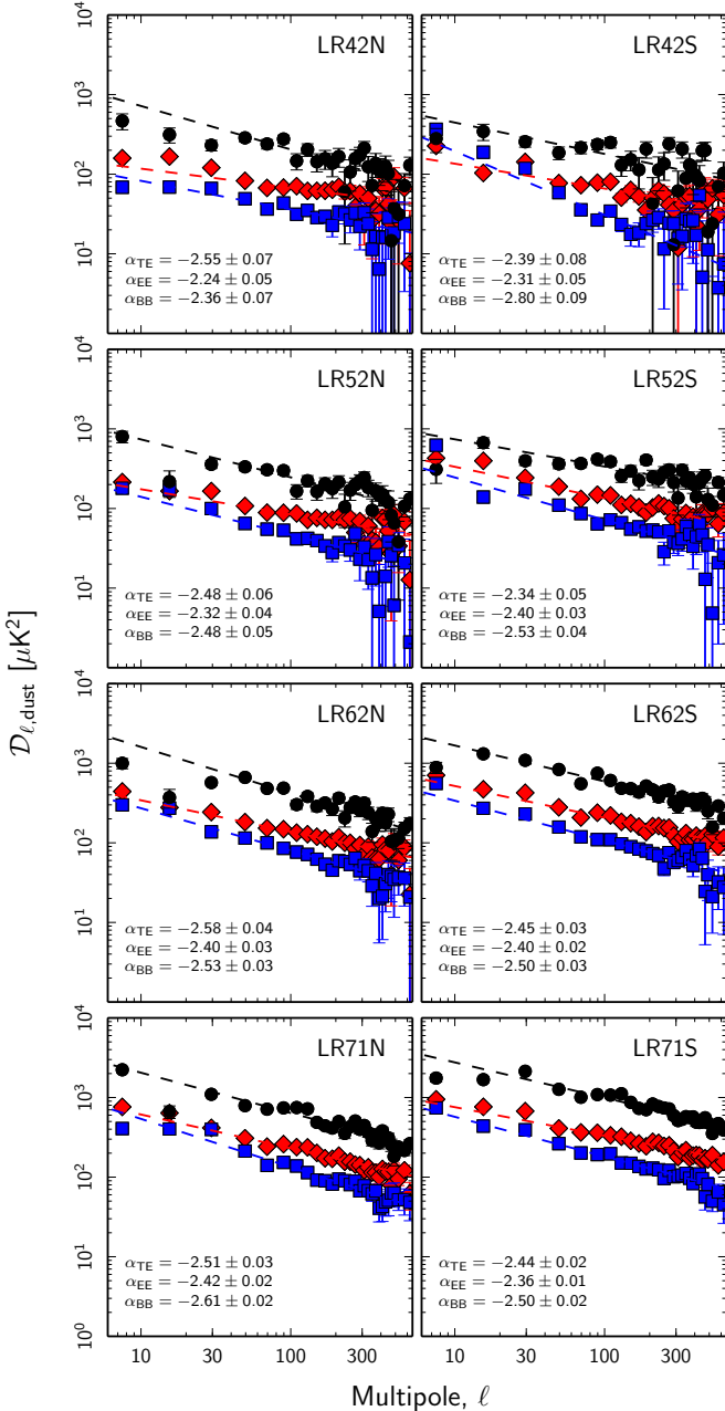
Fig. 2. Power spectra, as in Fig. 3, but for the northern and southern parts of the LR42, LR52, LR62, and LR71 regions.
