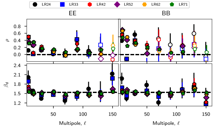
Fig. 9. Fit parameters \rho and \beta_d for E - and B -mode polarization versus multipole. Note the linear scale. Open symbols for \rho represent the cases where the synchrotron amplitude is compatible with zero, making it difficult to measure the correlation.
