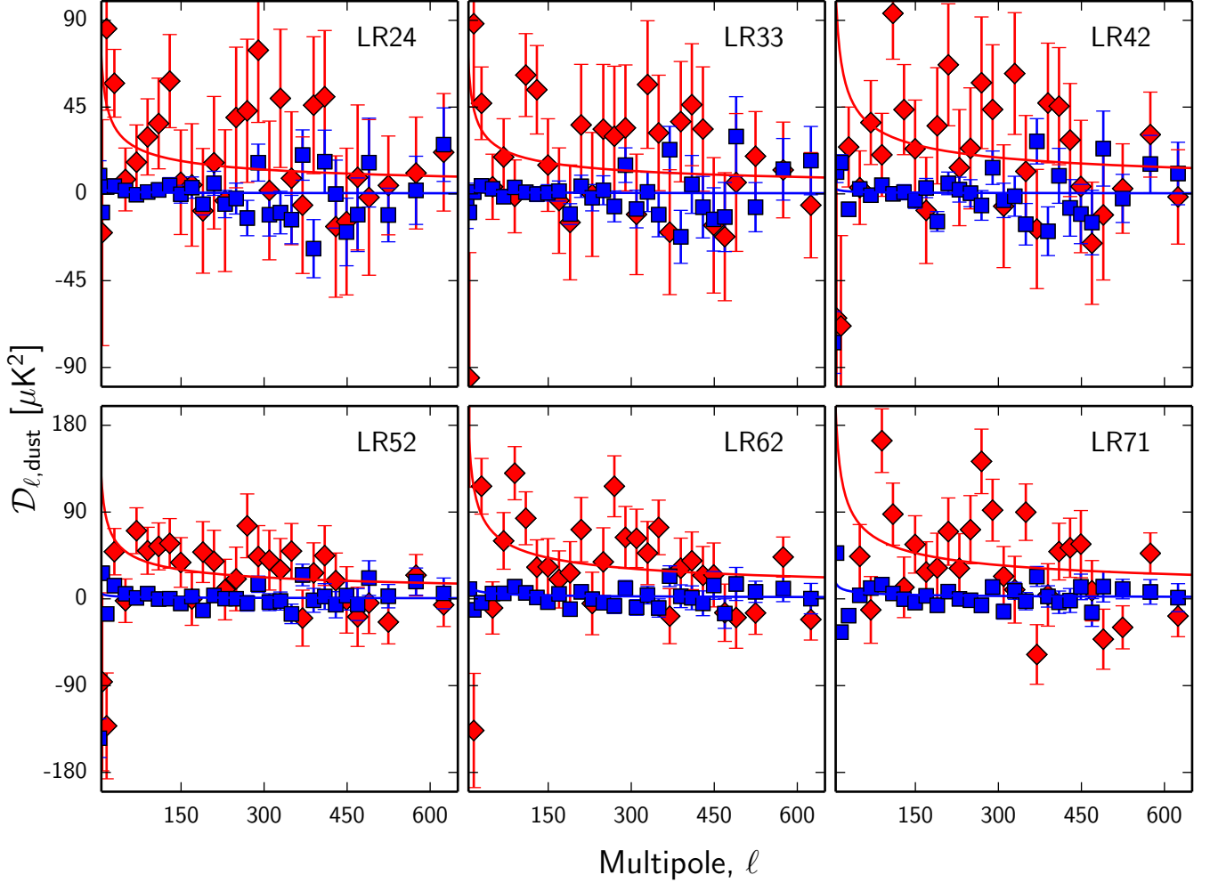
Fig. 5. Power spectra of TB (red diamonds) and EB (blue squares) at 353 GHz for the six sky regions. The error bars are derived from the E2E simulations. A power-law fit to the TB data (solid red line) reveals an overall positive TB signal, not seen in the E2E simulations. The EB power (solid blue line fit) is consistent with zero.
