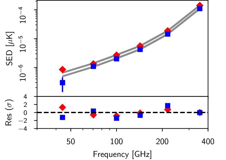
Fig. 13. Dust SEDs for E - and B -mode polarization derived from the SMICA component-separation procedure ( Planck Collaboration IV 2018 ). The two grey lines represent MBB fits to the E - (red diamonds) and B -mode (blue squares) data points with a temperature of 19.6 K. The polarization spectral index derived from the fits is \beta_d^P = 1.53 \pm 0.02 . The residuals to each fit, normalized to the 1\sigma data uncertainty, are plotted in the lower part of each panel.
