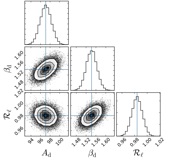
Fig. 15. Posterior distribution for each of the parameters of the spectral model with decorrelation given in Eq. (5), as obtained through the MCMC fitting algorithm for BB data points. The MCMC results illustrated here are for the LR62 region and the multipole range 50–160. Median values are A_d = 97.1 \pm 1.2 , \beta_d = 1.54 \pm 0.02 , and \mathcal{R}_\ell^{\text{BB}}(217, 353) = 0.984 \pm 0.008 .
