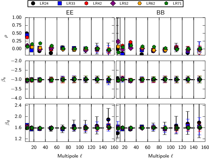
Fig. A.4. Results of the spectral fit to simulated data with uncertainties derived from the E2E simulated maps. Distinct symbols and colours represent the different sky regions (see top row). The dashed lines in plots of \beta_s and \beta_d are the input values of our sky model. We retrieve these input values without any bias. The sky model has a non-zero correlation between dust and synchrotron polarization at low \ell , which is consistent with the value of \rho found by fitting the simulated data.
