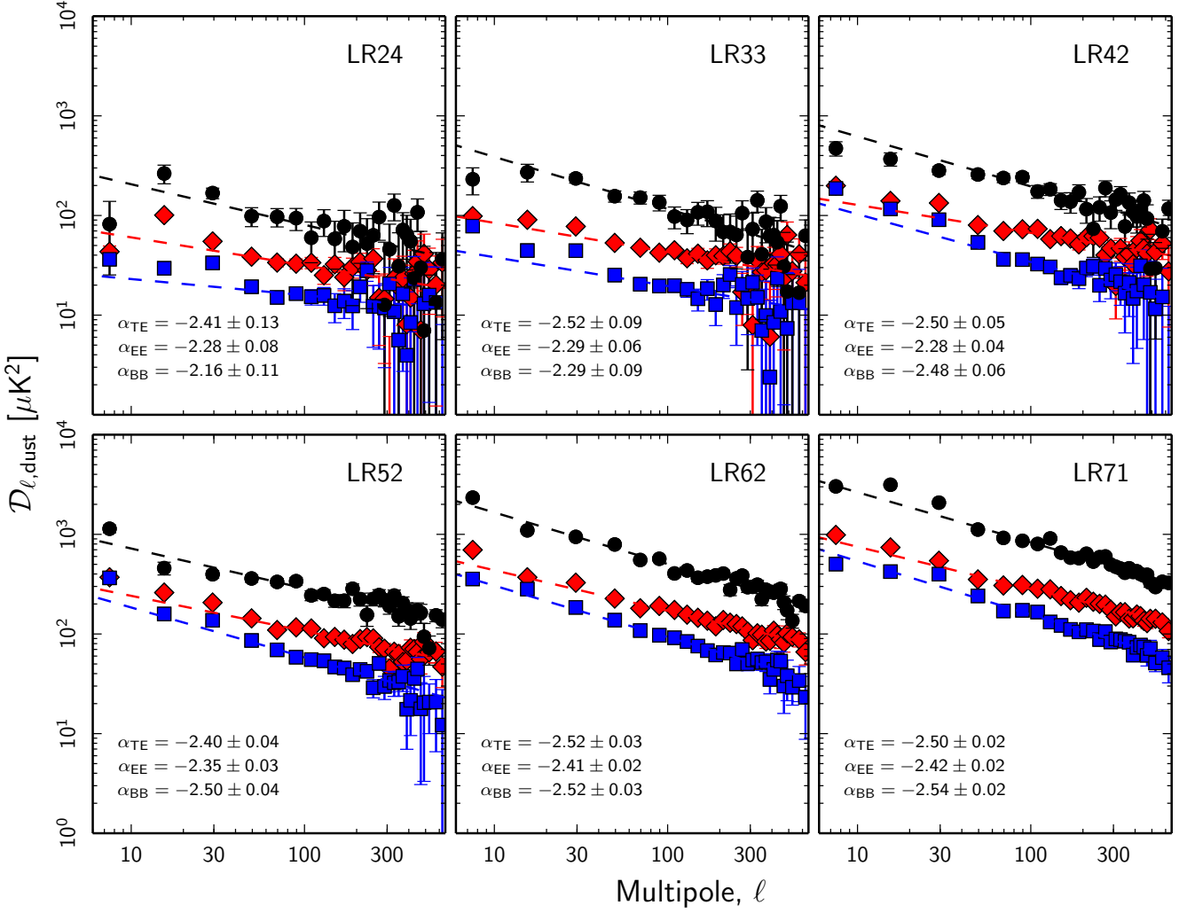
caption[J]CMB-corrected EE (red diamonds), BB (blue squares), and TE (black circles) power spectra at 353 GHz, for each of the six sky regions that we analyse. The dashed lines represent power-law fits to the data points from \ell = 40 to 600. The exponents of these fits, \alpha_{TE} , \alpha_{EE} , and \alpha_{BB} , appear on each panel.
