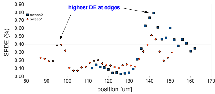
Figure 3.2: Measured SPDE over spatial position of a diffused guard ring device.
