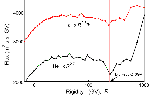
FIG. 1 (color online). PAMELA fluxes of He and protons. He (solid line) and protons (dashed line) are multiplied by R^{2.7} and R^{2.8}/5 , respectively (proton spectrum artificially reduced to emphasize its similarity with the He spectrum). Circles represent PAMELA points adopted from Supplemental Material for [9]. The sharp rise of the He beyond R \approx 800 GV is likely to be associated with growing errors, since it does not match with the ATIC-2 and CREAM [11,16] data at R \gtrsim 10^3 GV. The “zig-zags” on each spectrum (also present at lower energies) are well within the error bars (not shown here).
