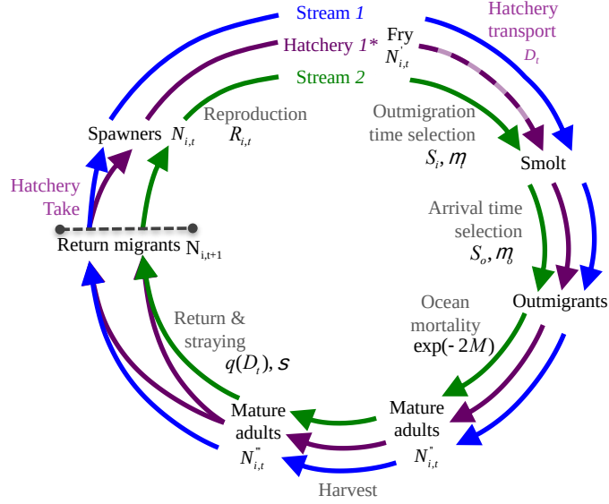
Figure 1. Outline of the model dynamics
