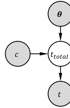
Figure 1. Graphical model (observer perspective)
