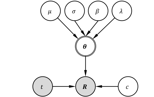
Figure 2. Graphical model (researcher perspective)
