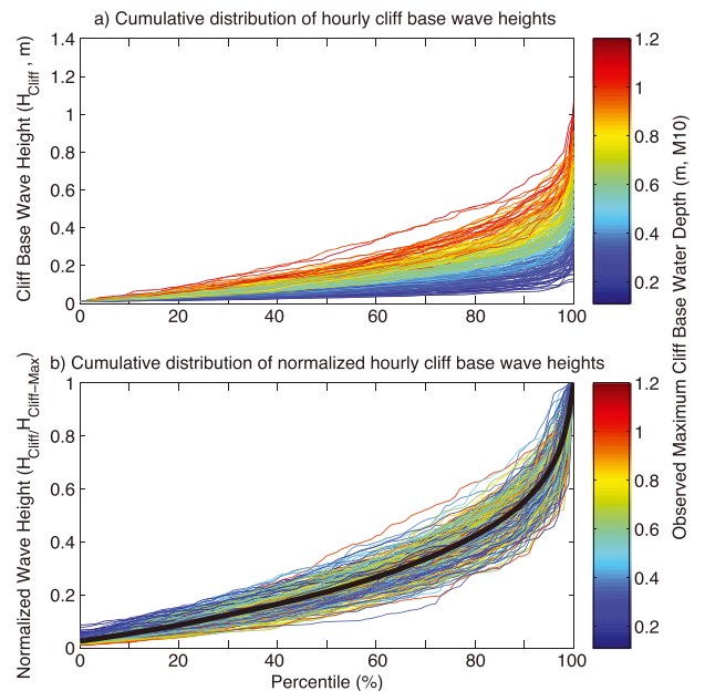
Figure 6. Cumulative distribution of (a) cliff base impact wave heights ( H_{Cliff} ) during each hour, and (b) cliff base impact wave heights normalized by maximum hourly cliff base wave height ( H_{Cliff-Max} ) during each hour and the overall mean (thick black line). Colors are observed maximum hourly cliff base water depth (M10).
