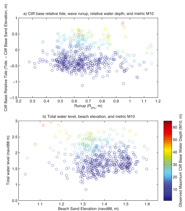
Figure 8. Impact metric M10 (observed maximum depth at cliff base, color bar) versus (horizontal and vertical axes, respectively) (a) cliff base relative tide (tide level minus beach elevation) and wave-induced runup, (b) modeled total water level and beach sand elevation. Only hours with M10 > 0 are shown.
