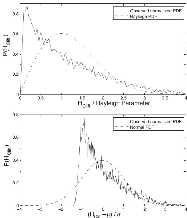
Figure 5. Normalized ensemble-average observed cliff base wave ( H_{Cliff} ) distribution (for hours with at least 100 waves used) compared with standard (top) Rayleigh and (bottom) Normal distributions.
