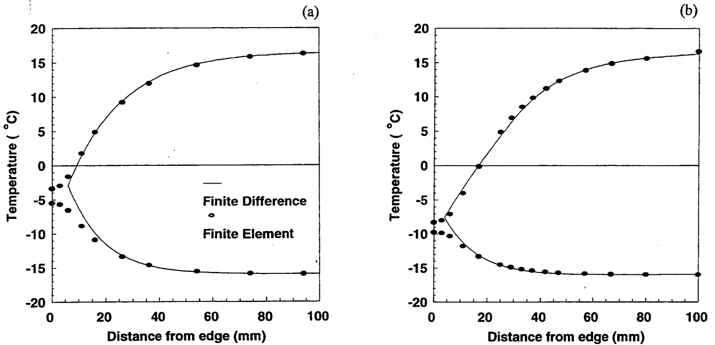
Figure 7 Finite difference and finite element modeling results for a vacuum glazing with (a) an uninsulated edge seal, and (b) an insulated edge seal.
