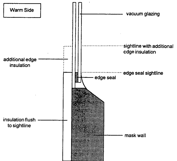
Figure 3 Cross sectional schematic of the vacuum glazing edge-of-glass region as mounted for infrared thermographic testing
