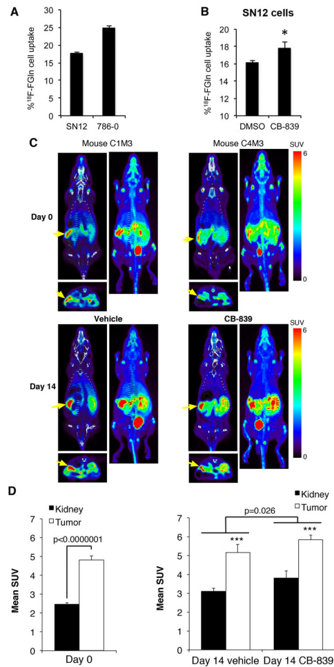
Fig. 6. 18 F-FGln cell uptake and 4-[ 18 F]fluoroglutamine-PET imaging
